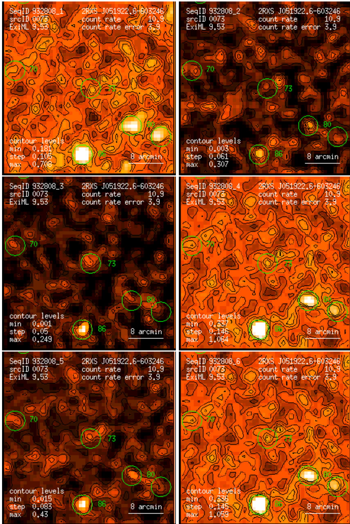
Figure 73: RASS 932808: detection 0073: band rate images, Gaussian filter: (1) PSPC channels 11 – 41, (2) 52 – 90, (3) 91 – 201, (4) 11 – 235, (5) 52 – 201, (6) 11 – 201. Broad band rates in counts/ks. Band rate contour levels in counts/ks/arcmin 2 .
