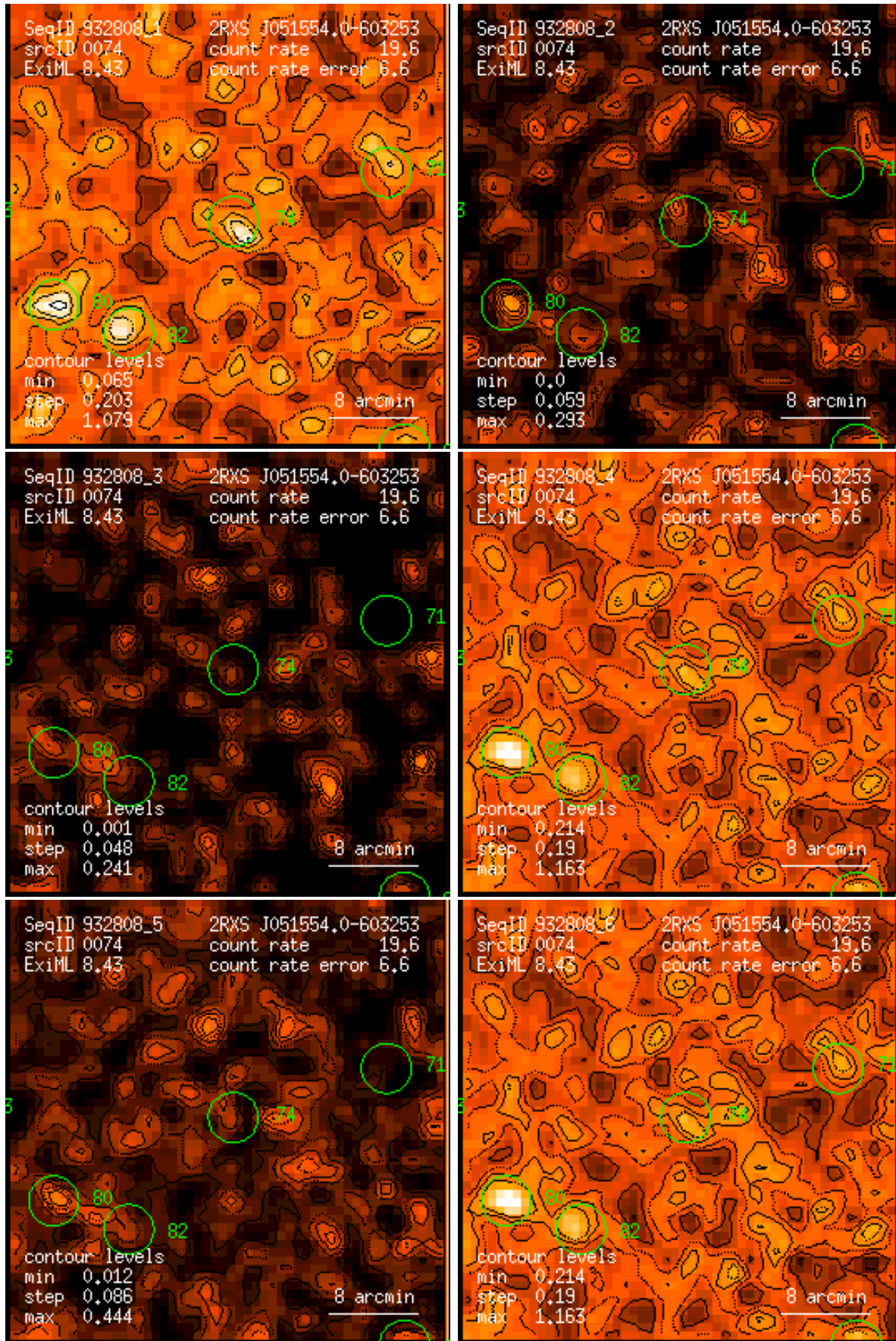
Figure 74: RASS 932808: detection 0074: band rate images, Gaussian filter: (1) PSPC channels 11 – 41, (2) 52 – 90, (3) 91 – 201, (4) 11 – 235, (5) 52 – 201, (6) 11 – 201. Broad band rates in counts/ks. Band rate contour levels in counts/ks/arcmin 2 .
