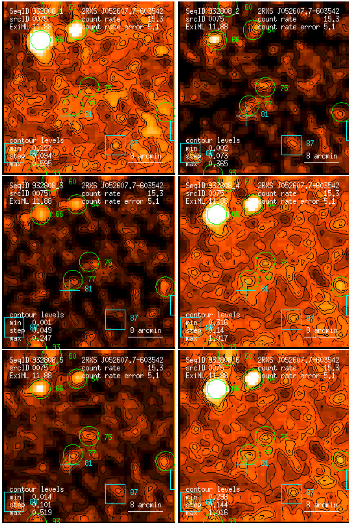
Figure 75: RASS 932808: detection 0075: band rate images, Gaussian filter: (1) PSPC channels 11 – 41, (2) 52 – 90, (3) 91 – 201, (4) 11 – 235, (5) 52 – 201, (6) 11 – 201. Broad band rates in counts/ks. Band rate contour levels in counts/ks/arcmin 2 .
