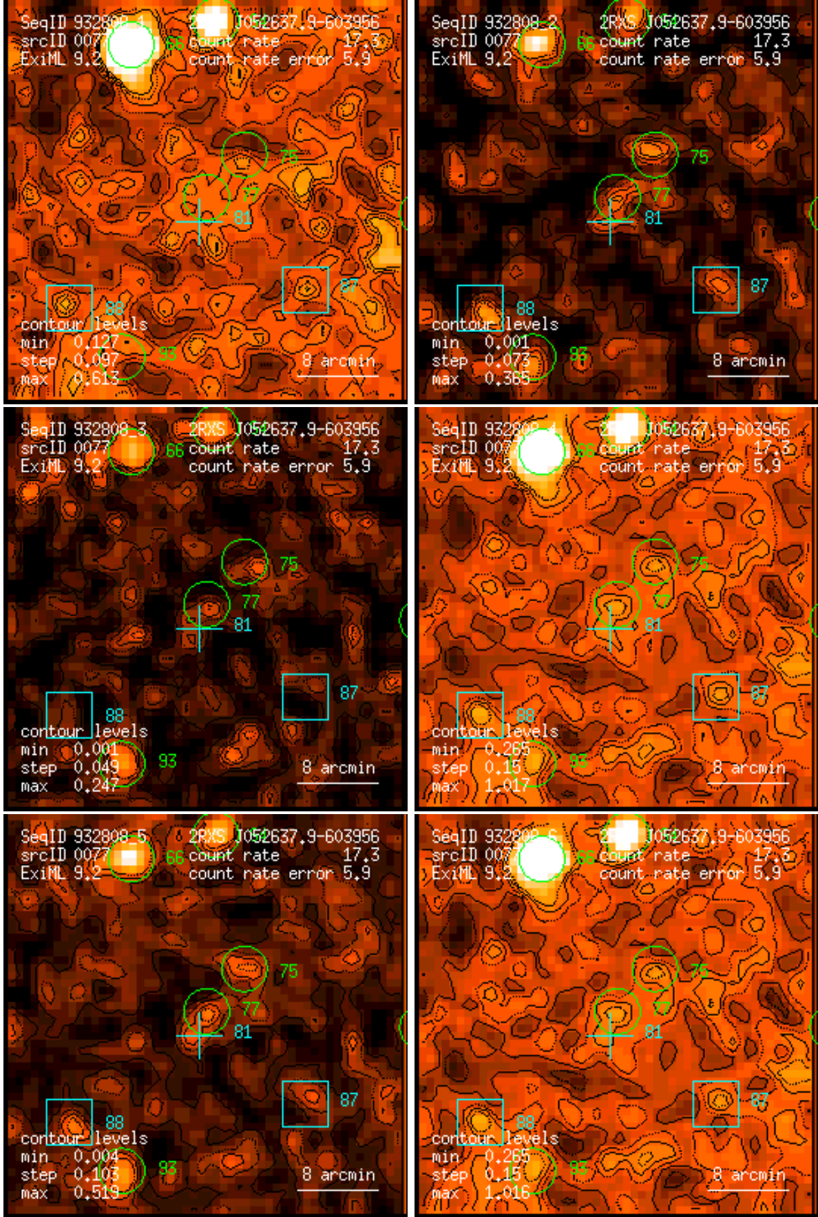
Figure 77: RASS 932808: detection 0077: band rate images, Gaussian filter: (1) PSPC channels 11 – 41, (2) 52 – 90, (3) 91 – 201, (4) 11 – 235, (5) 52 – 201, (6) 11 – 201. Broad band rates in counts/ks. Band rate contour levels in counts/ks/arcmin 2 .
