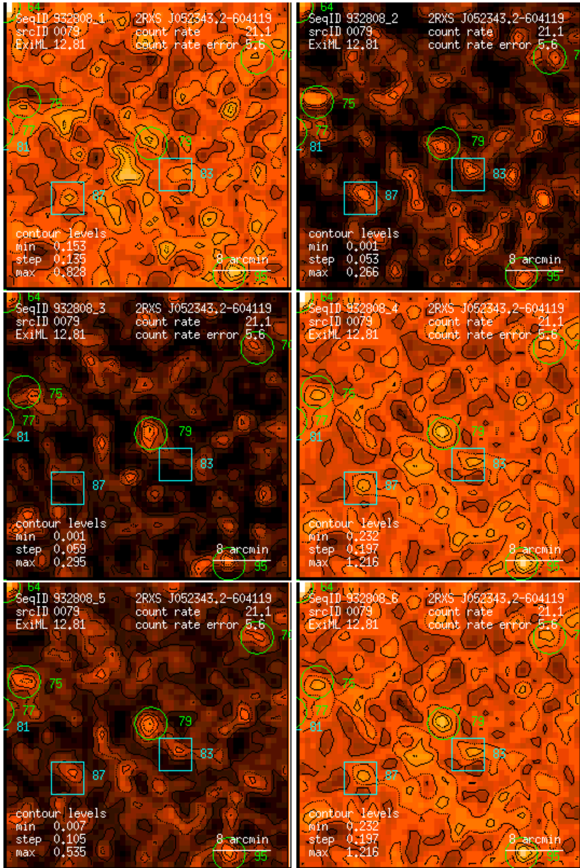
Figure 79: RASS 932808: detection 0079: band rate images, Gaussian filter: (1) PSPC channels 11 – 41, (2) 52 – 90, (3) 91 – 201, (4) 11 – 235, (5) 52 – 201, (6) 11 – 201. Broad band rates in counts/ks. Band rate contour levels in counts/ks/arcmin 2 .
