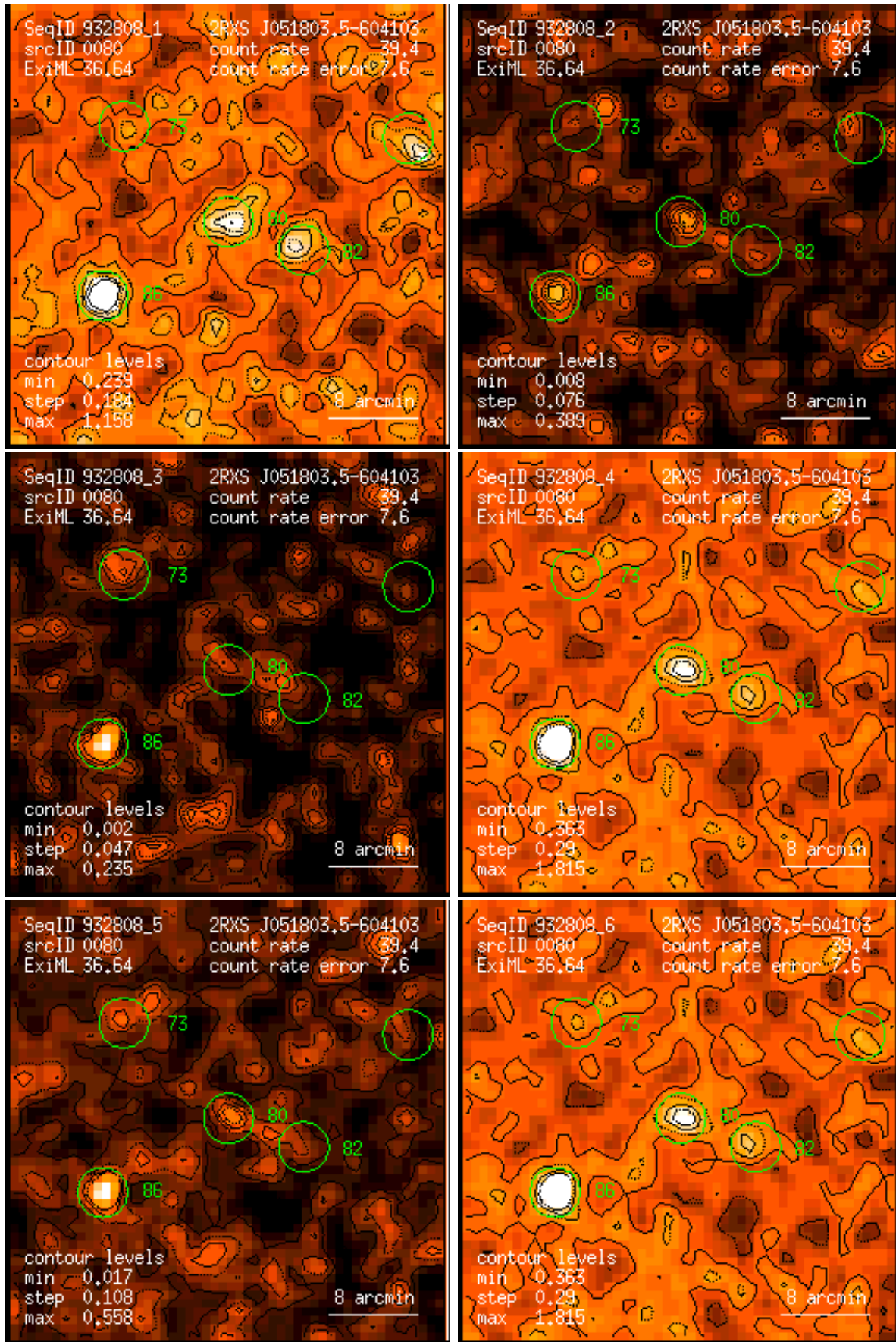
Figure 80: RASS 932808: detection 0080: band rate images, Gaussian filter: (1) PSPC channels 11 – 41, (2) 52 – 90, (3) 91 – 201, (4) 11 – 235, (5) 52 – 201, (6) 11 – 201. Broad band rates in counts/ks. Band rate contour levels in counts/ks/arcmin 2 .
