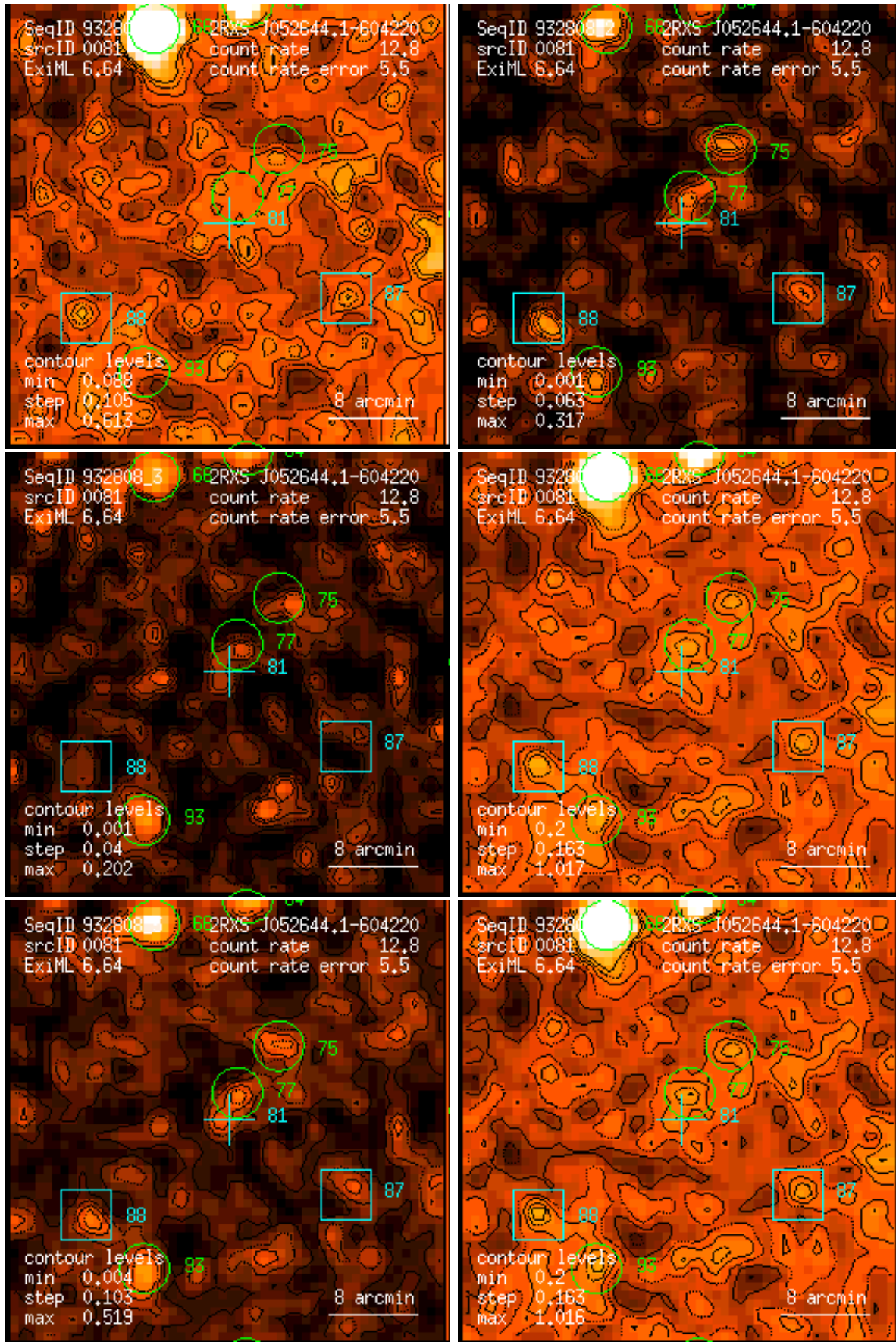
Figure 81: RASS 932808: detection 0081: band rate images, Gaussian filter: (1) PSPC channels 11 – 41, (2) 52 – 90, (3) 91 – 201, (4) 11 – 235, (5) 52 – 201, (6) 11 – 201. Broad band rates in counts/ks. Band rate contour levels in counts/ks/arcmin 2 .
