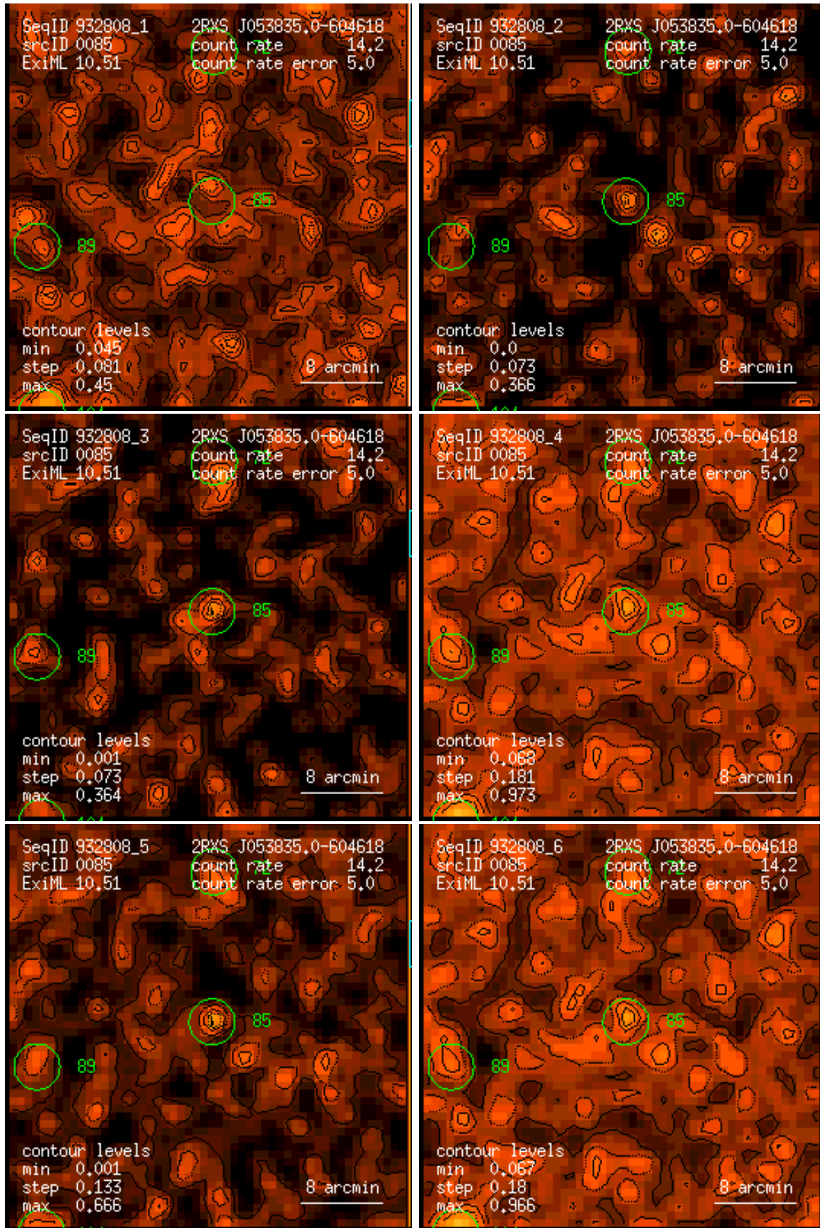
Figure 85: RASS 932808: detection 0085: band rate images, Gaussian filter: (1) PSPC channels 11 – 41, (2) 52 – 90, (3) 91 – 201, (4) 11 – 235, (5) 52 – 201, (6) 11 – 201. Broad band rates in counts/ks. Band rate contour levels in counts/ks/arcmin 2 .
