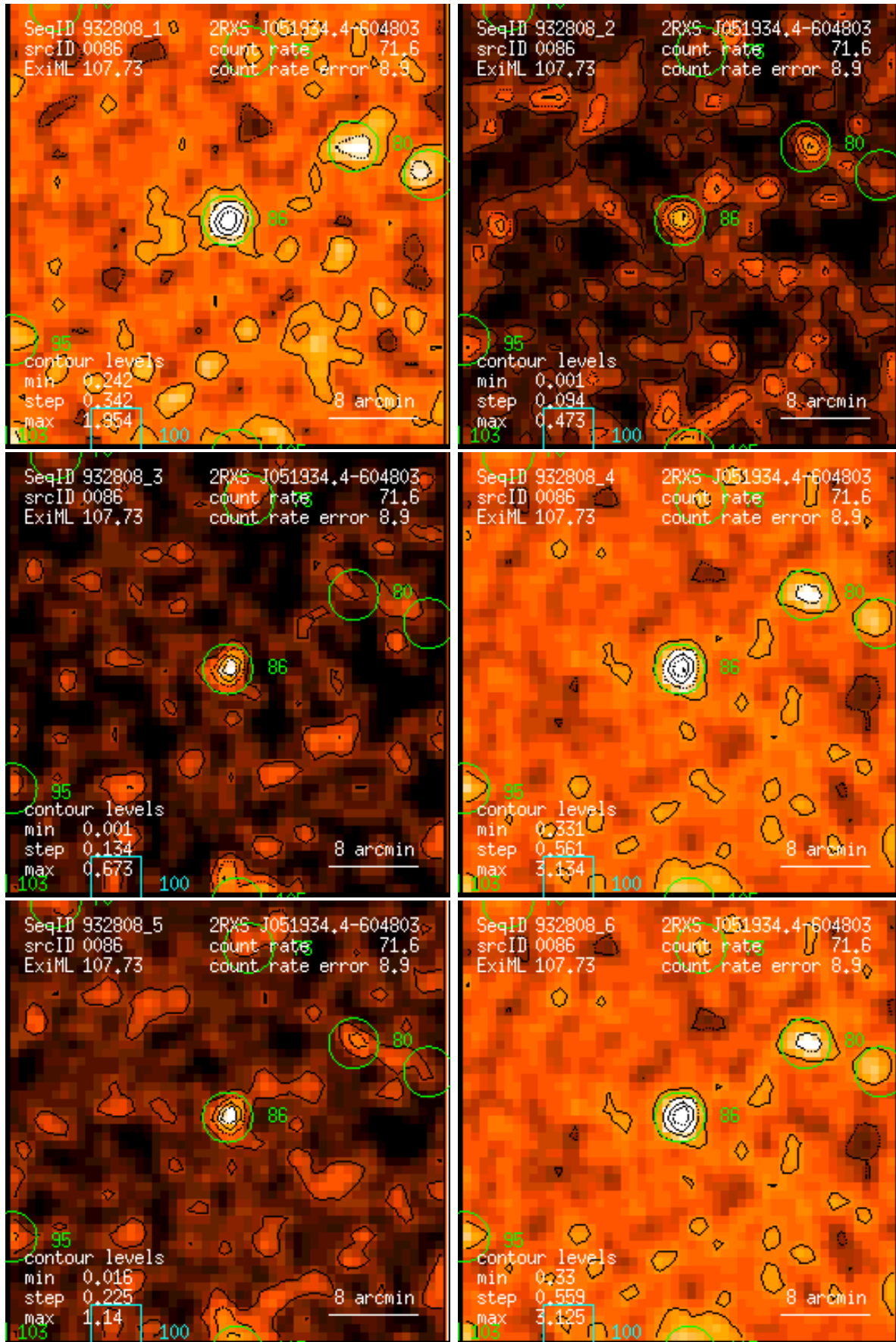
Figure 86: RASS 932808: detection 0086: band rate images, Gaussian filter: (1) PSPC channels 11 – 41, (2) 52 – 90, (3) 91 – 201, (4) 11 – 235, (5) 52 – 201, (6) 11 – 201. Broad band rates in counts/ks. Band rate contour levels in counts/ks/arcmin 2 .
