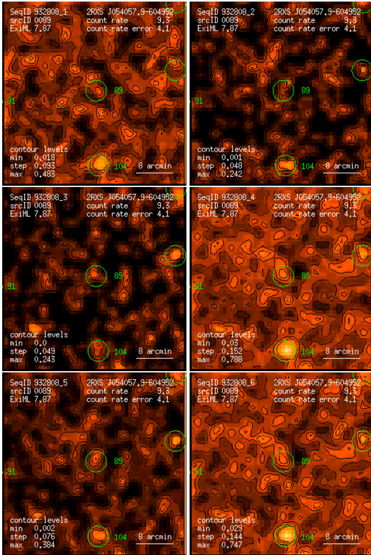
Figure 89: RASS 932808: detection 0089: band rate images, Gaussian filter: (1) PSPC channels 11 – 41, (2) 52 – 90, (3) 91 – 201, (4) 11 – 235, (5) 52 – 201, (6) 11 – 201. Broad band rates in counts/ks. Band rate contour levels in counts/ks/arcmin 2 .
