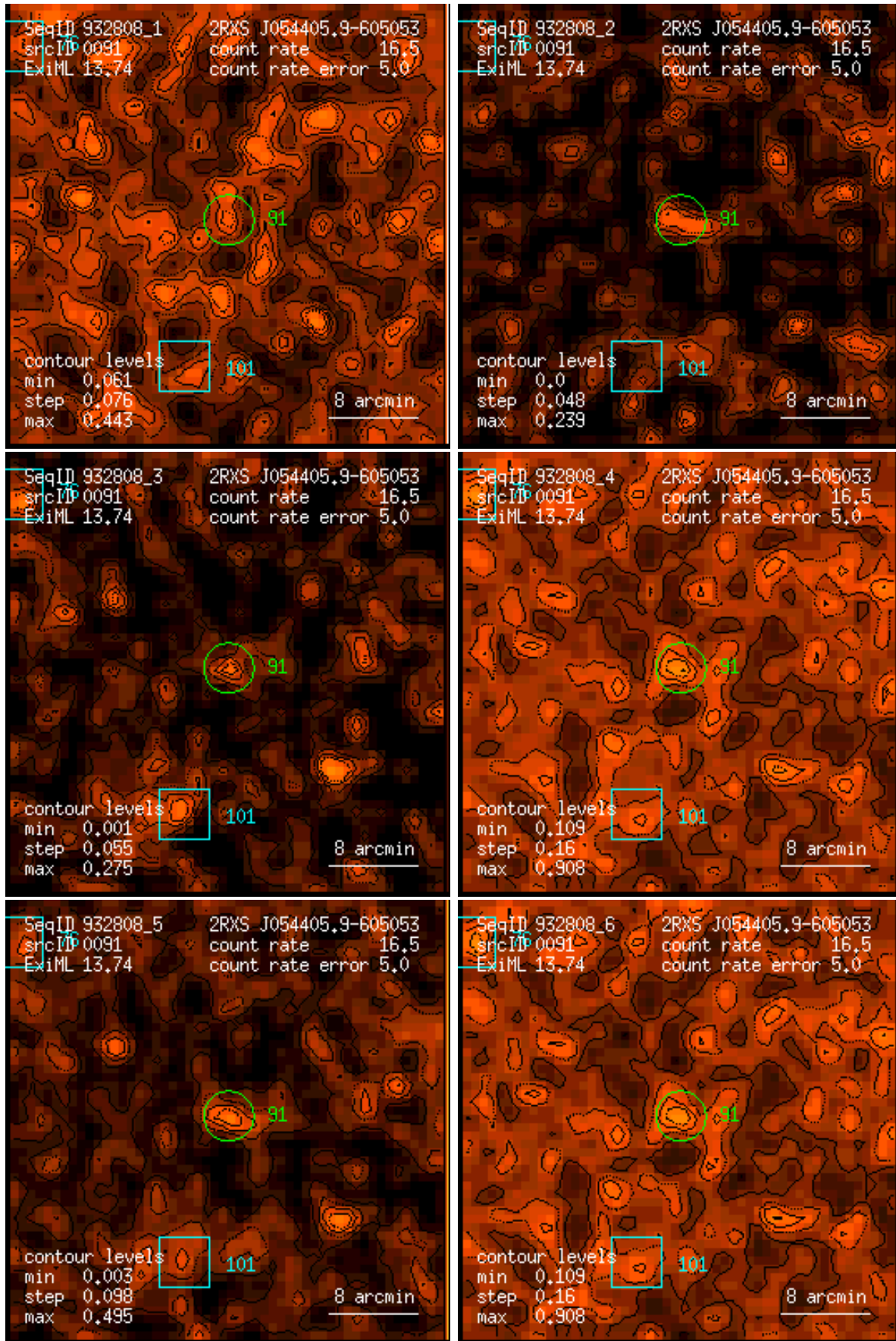
Figure 91: RASS 932808: detection 0091: band rate images, Gaussian filter: (1) PSPC channels 11 – 41, (2) 52 – 90, (3) 91 – 201, (4) 11 – 235, (5) 52 – 201, (6) 11 – 201. Broad band rates in counts/ks. Band rate contour levels in counts/ks/arcmin 2 .
