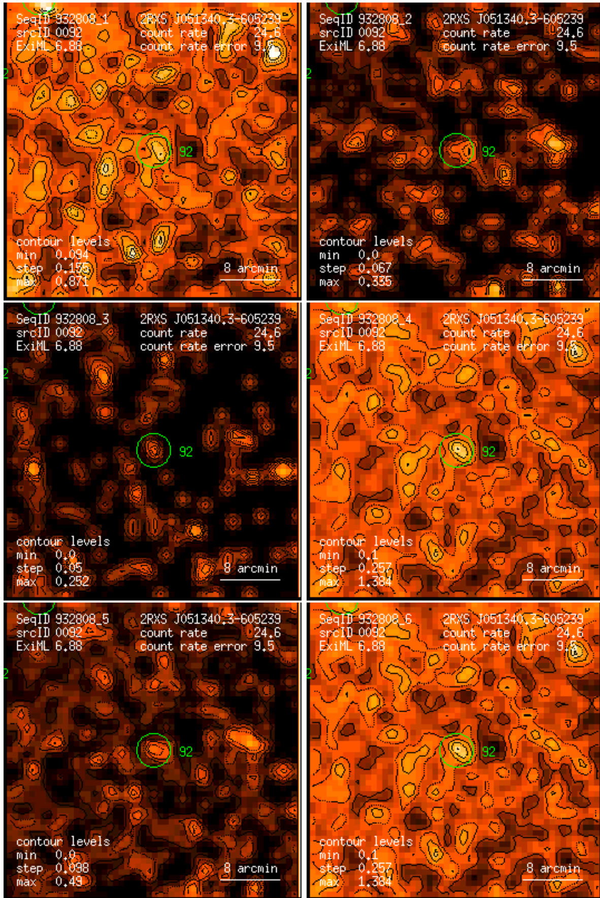
Figure 92: RASS 932808: detection 0092: band rate images, Gaussian filter: (1) PSPC channels 11 – 41, (2) 52 – 90, (3) 91 – 201, (4) 11 – 235, (5) 52 – 201, (6) 11 – 201. Broad band rates in counts/ks. Band rate contour levels in counts/ks/arcmin 2 .
