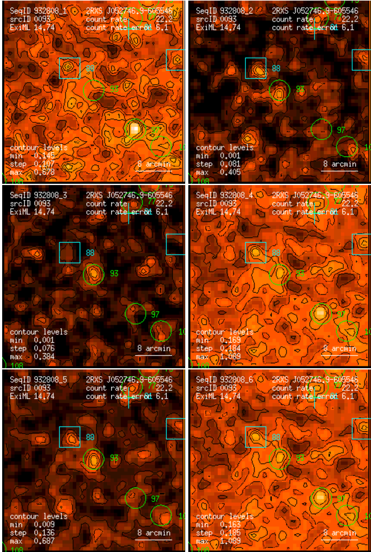
Figure 93: RASS 932808: detection 0093: band rate images, Gaussian filter: (1) PSPC channels 11 – 41, (2) 52 – 90, (3) 91 – 201, (4) 11 – 235, (5) 52 – 201, (6) 11 – 201. Broad band rates in counts/ks. Band rate contour levels in counts/ks/arcmin 2 .
