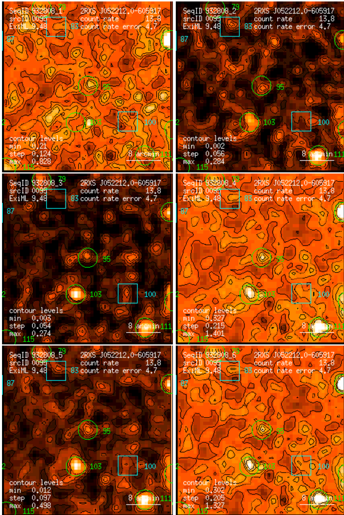
Figure 95: RASS 932808: detection 0095: band rate images, Gaussian filter: (1) PSPC channels 11 – 41, (2) 52 – 90, (3) 91 – 201, (4) 11 – 235, (5) 52 – 201, (6) 11 – 201. Broad band rates in counts/ks. Band rate contour levels in counts/ks/arcmin 2 .
