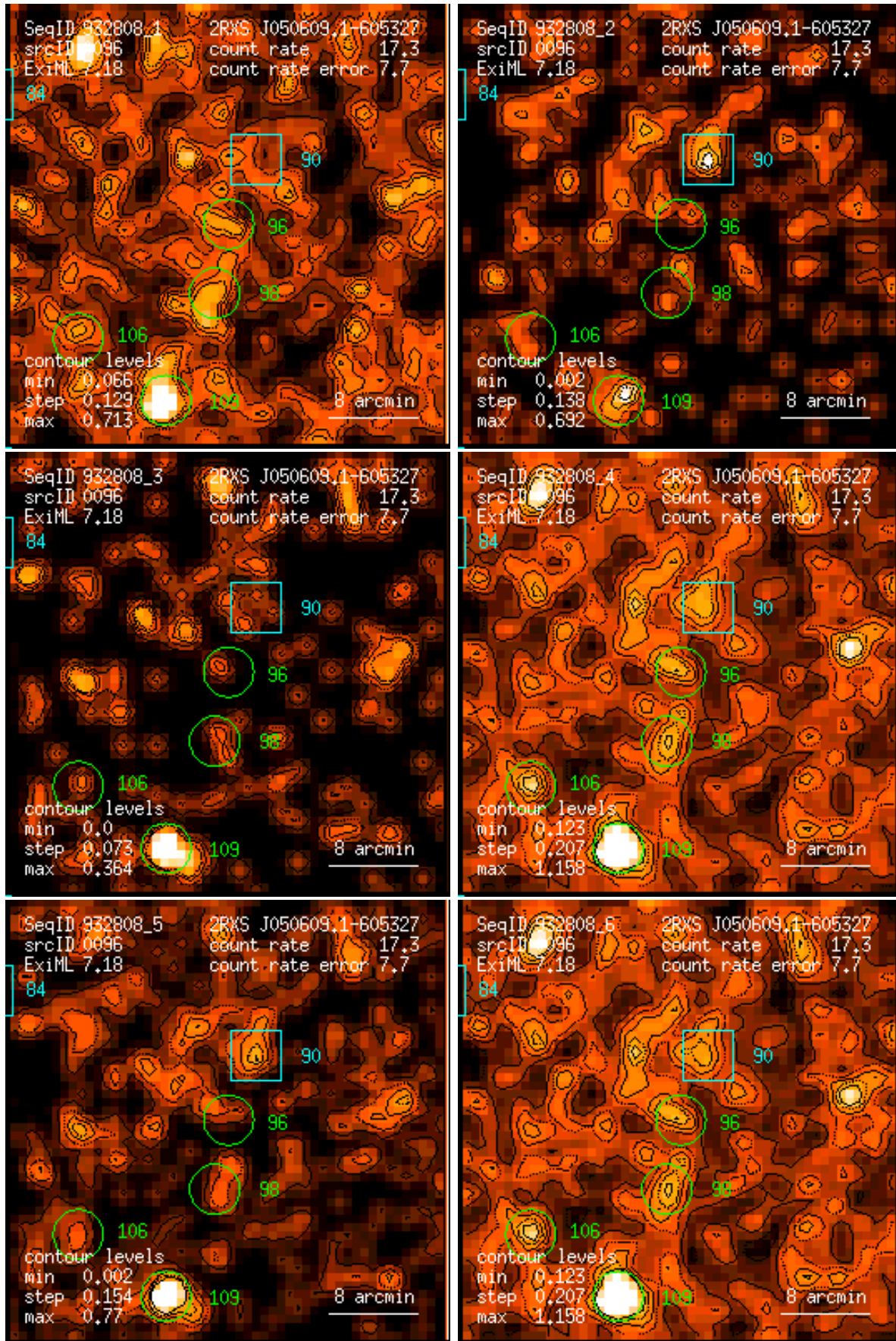
Figure 96: RASS 932808: detection 0096: band rate images, Gaussian filter: (1) PSPC channels 11 – 41, (2) 52 – 90, (3) 91 – 201, (4) 11 – 235, (5) 52 – 201, (6) 11 – 201. Broad band rates in counts/ks. Band rate contour levels in counts/ks/arcmin 2 .
