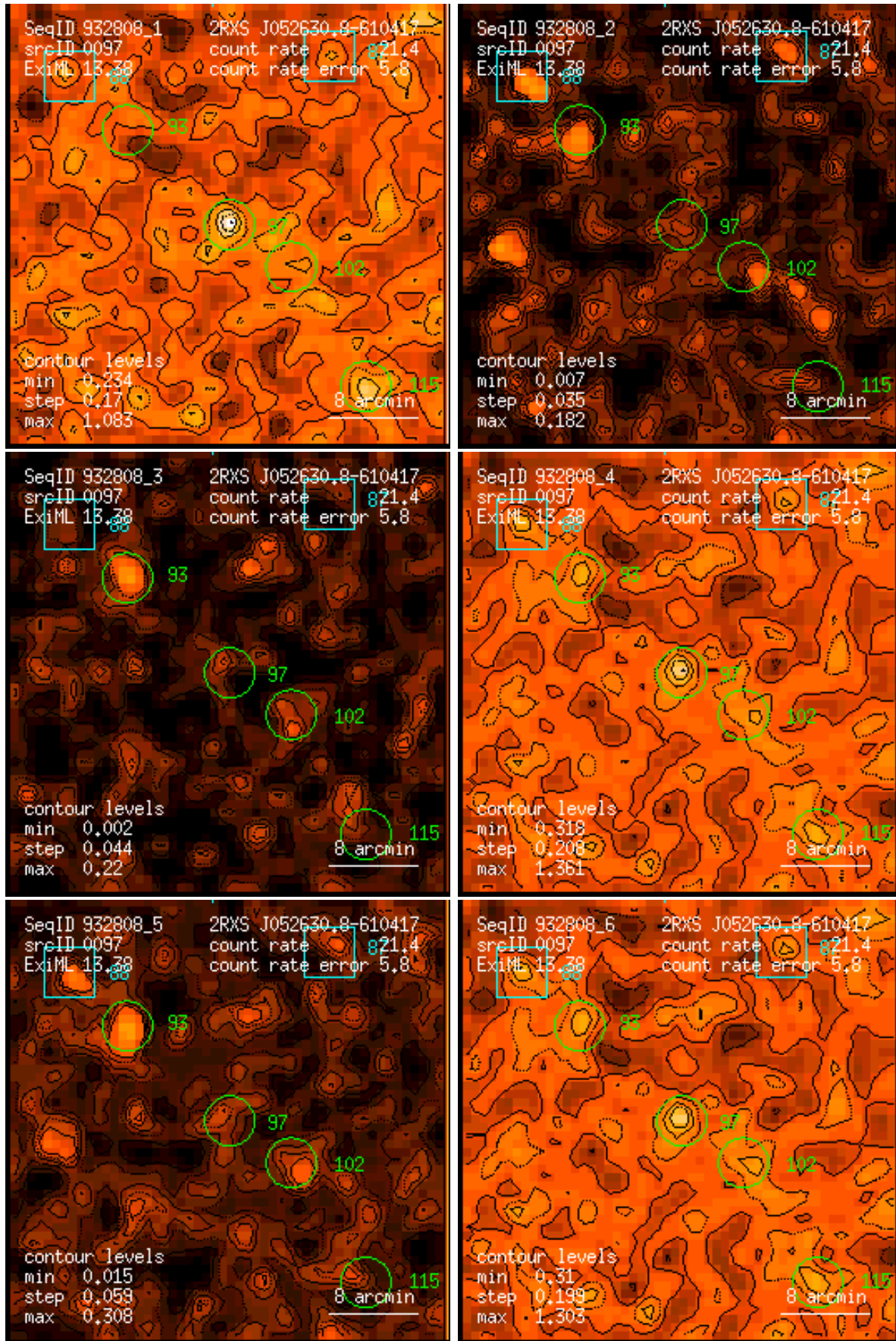
Figure 97: RASS 932808: detection 0097: band rate images, Gaussian filter: (1) PSPC channels 11 – 41, (2) 52 – 90, (3) 91 – 201, (4) 11 – 235, (5) 52 – 201, (6) 11 – 201. Broad band rates in counts/ks. Band rate contour levels in counts/ks/arcmin 2 .
