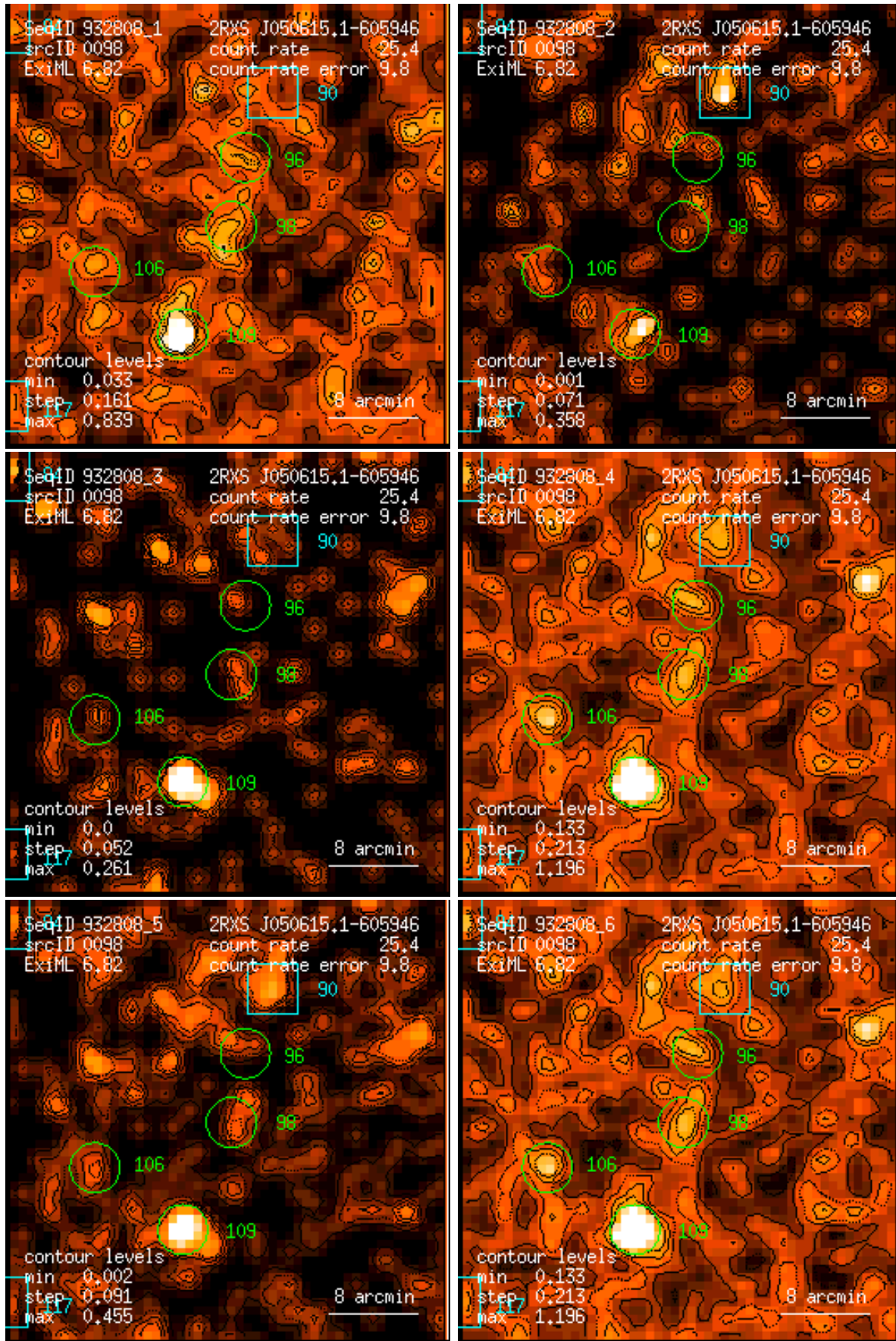
Figure 98: RASS 932808: detection 0098: band rate images, Gaussian filter: (1) PSPC channels 11 – 41, (2) 52 – 90, (3) 91 – 201, (4) 11 – 235, (5) 52 – 201, (6) 11 – 201. Broad band rates in counts/ks. Band rate contour levels in counts/ks/arcmin 2 .
