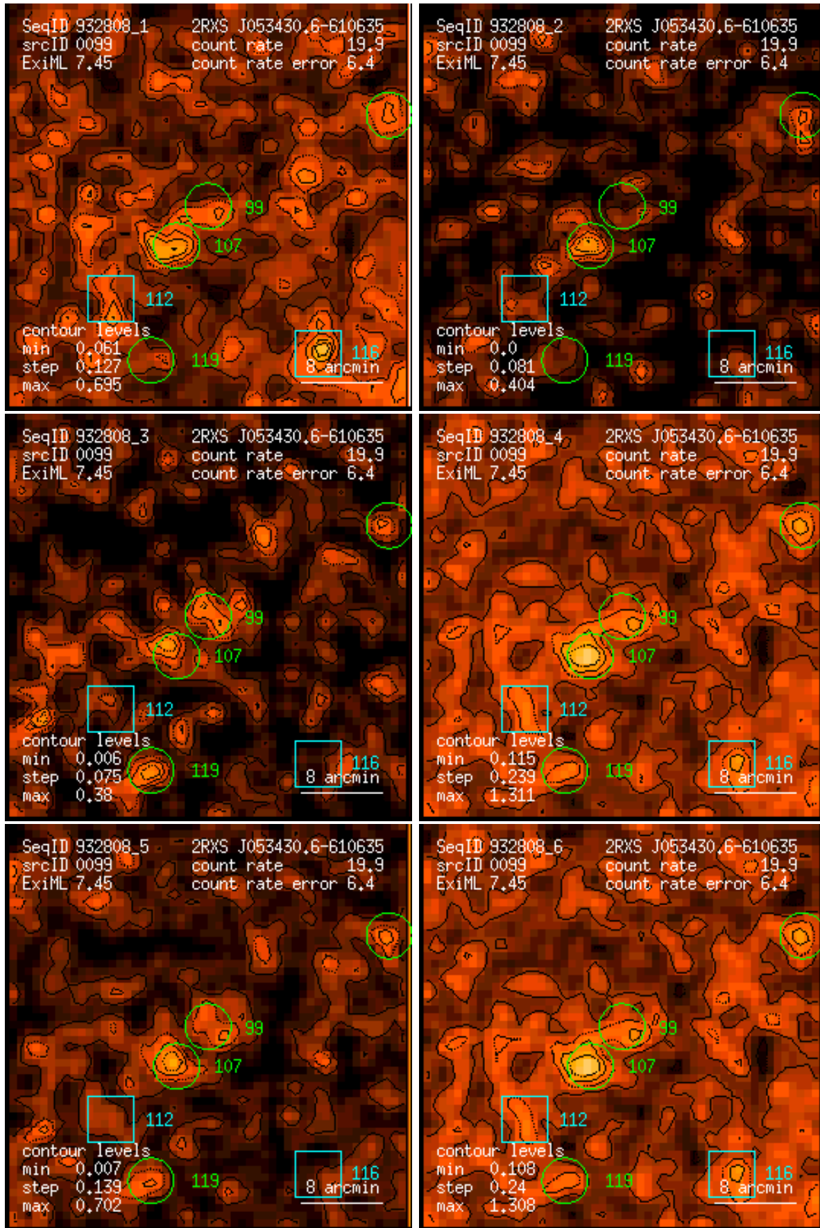
Figure 99: RASS 932808: detection 0099: band rate images, Gaussian filter: (1) PSPC channels 11 – 41, (2) 52 – 90, (3) 91 – 201, (4) 11 – 235, (5) 52 – 201, (6) 11 – 201. Broad band rates in counts/ks. Band rate contour levels in counts/ks/arcmin 2 .
