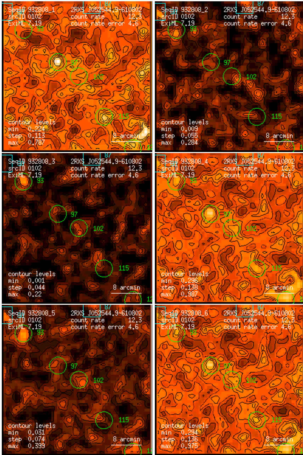
Figure 102: RASS 932808: detection 0102: band rate images, Gaussian filter: (1) PSPC channels 11 – 41, (2) 52 – 90, (3) 91 – 201, (4) 11 – 235, (5) 52 – 201, (6) 11 – 201. Broad band rates in counts/ks. Band rate contour levels in counts/ks/arcmin 2 .
