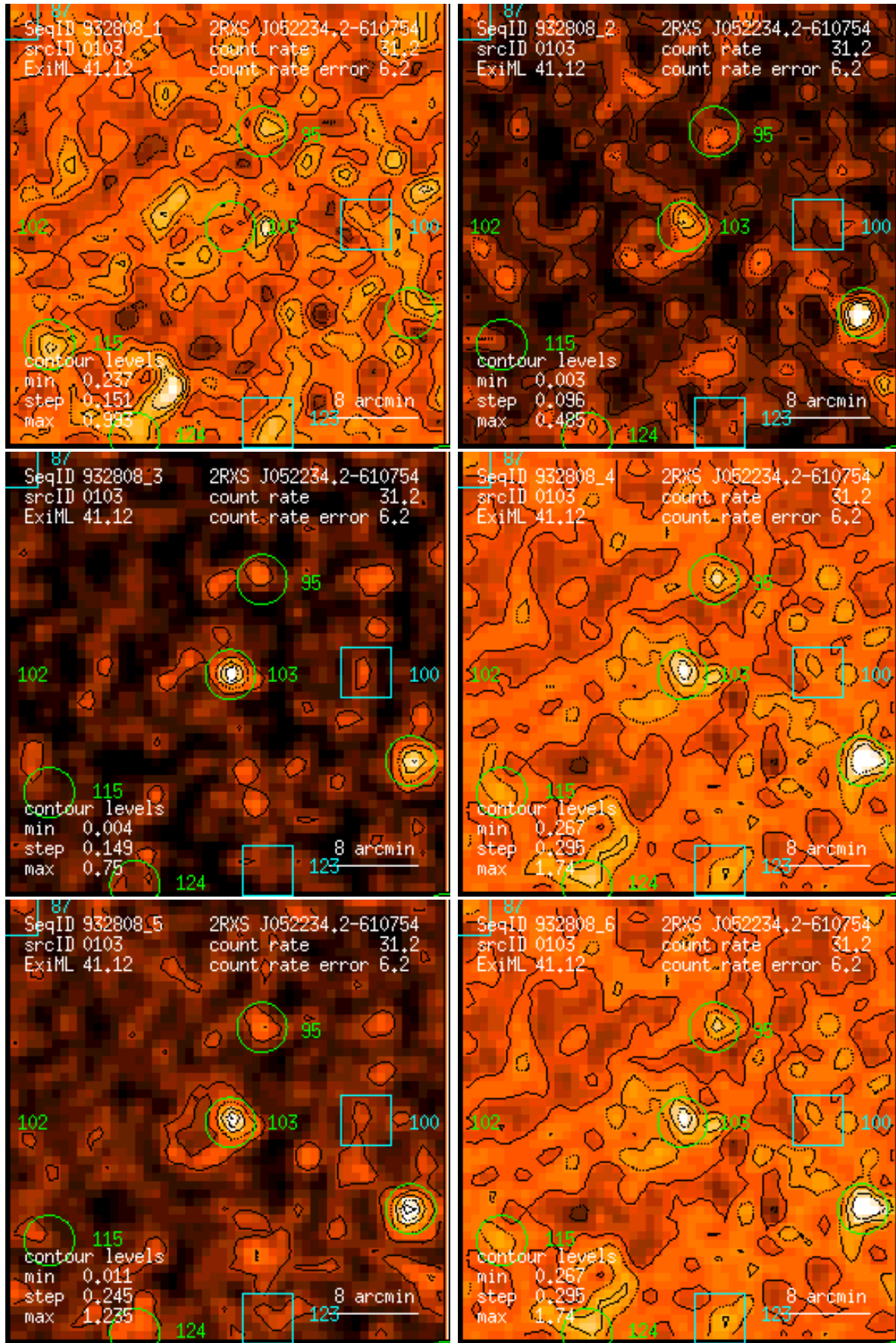
Figure 103: RASS 932808: detection 0103: band rate images, Gaussian filter: (1) PSPC channels 11 – 41, (2) 52 – 90, (3) 91 – 201, (4) 11 – 235, (5) 52 – 201, (6) 11 – 201. Broad band rates in counts/ks. Band rate contour levels in counts/ks/arcmin 2 .
