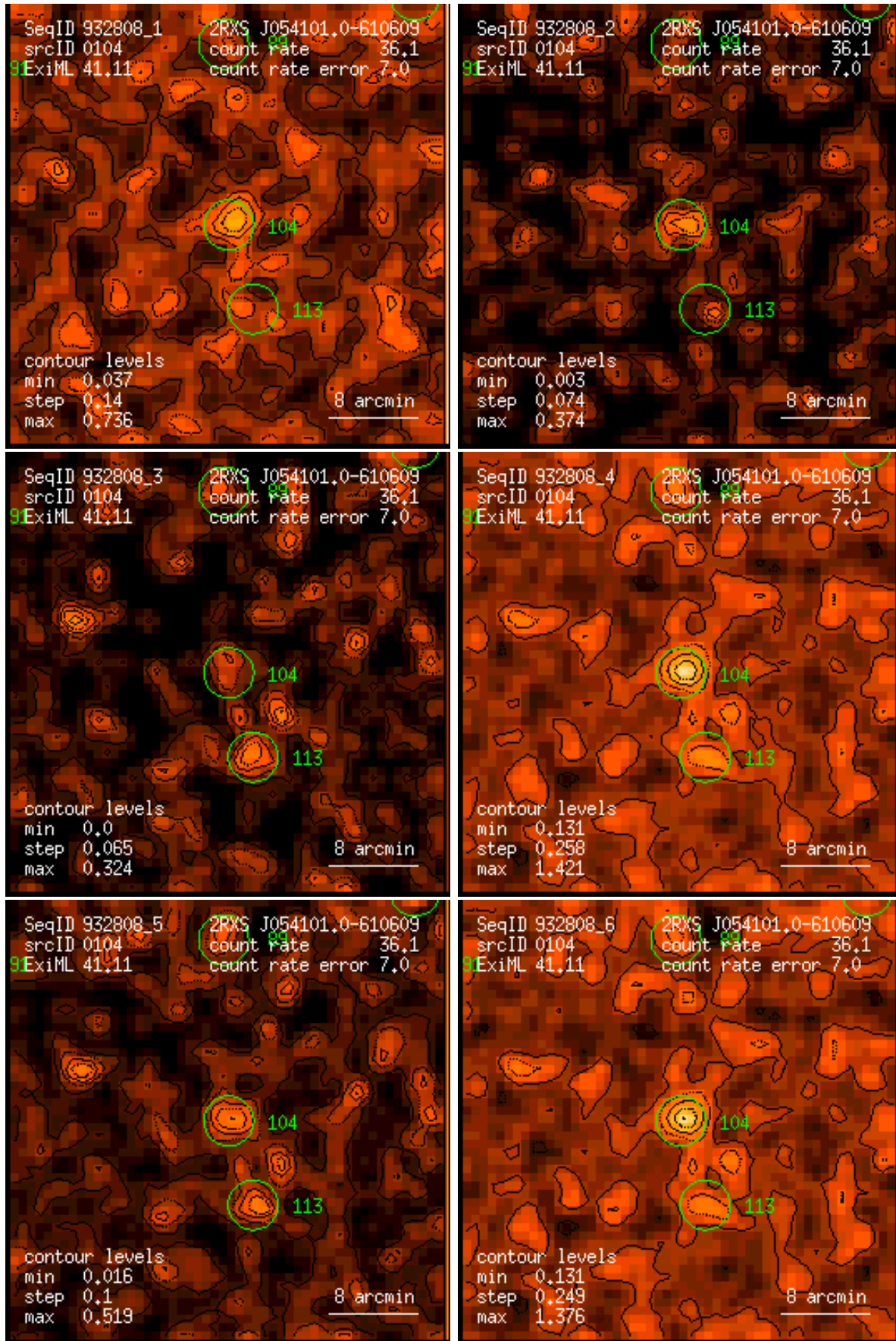
Figure 104: RASS 932808: detection 0104: band rate images, Gaussian filter: (1) PSPC channels 11 – 41, (2) 52 – 90, (3) 91 – 201, (4) 11 – 235, (5) 52 – 201, (6) 11 – 201. Broad band rates in counts/ks. Band rate contour levels in counts/ks/arcmin 2 .
