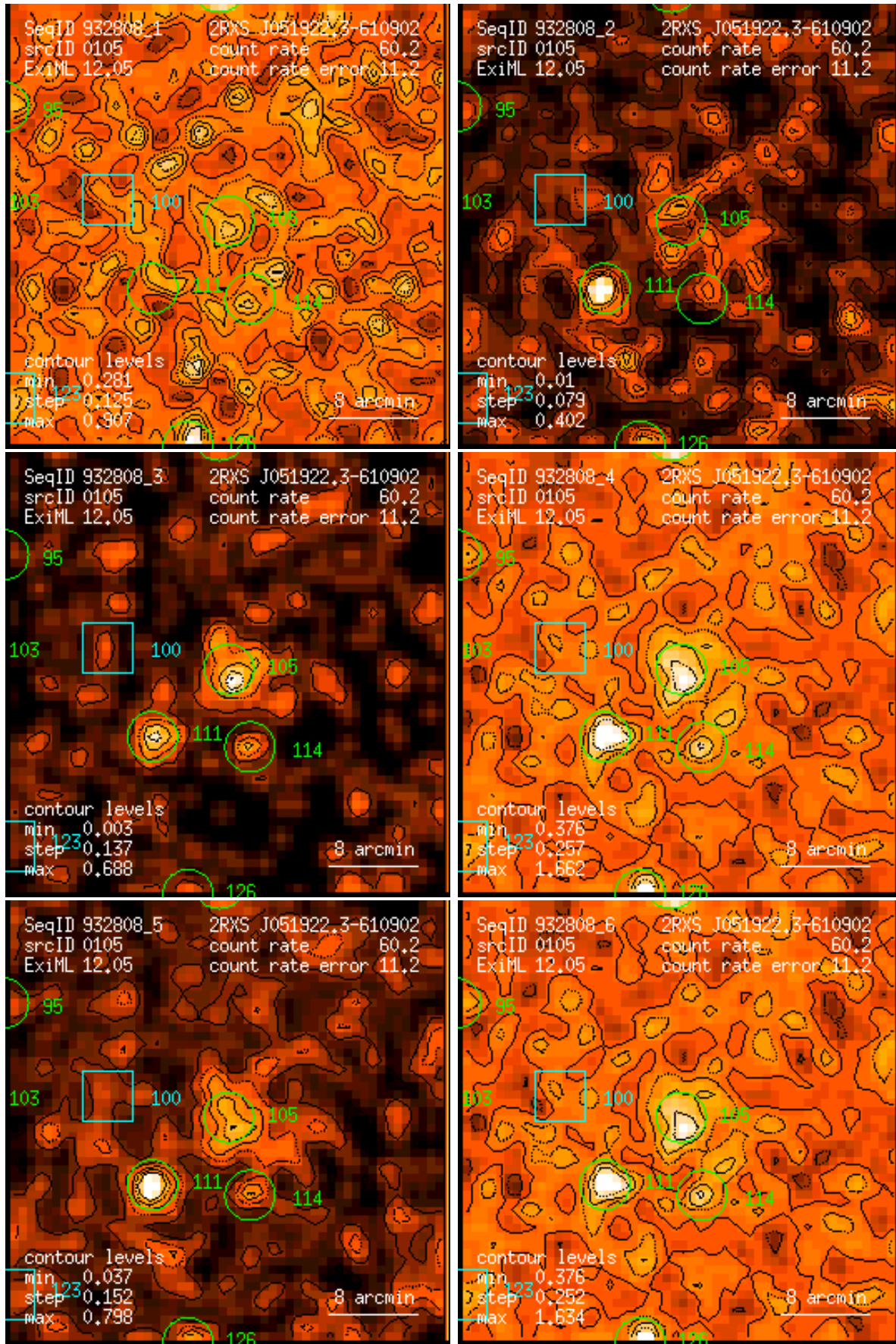
Figure 105: RASS 932808: detection 0105: band rate images, Gaussian filter: (1) PSPC channels 11 – 41, (2) 52 – 90, (3) 91 – 201, (4) 11 – 235, (5) 52 – 201, (6) 11 – 201. Broad band rates in counts/ks. Band rate contour levels in counts/ks/arcmin 2 .
