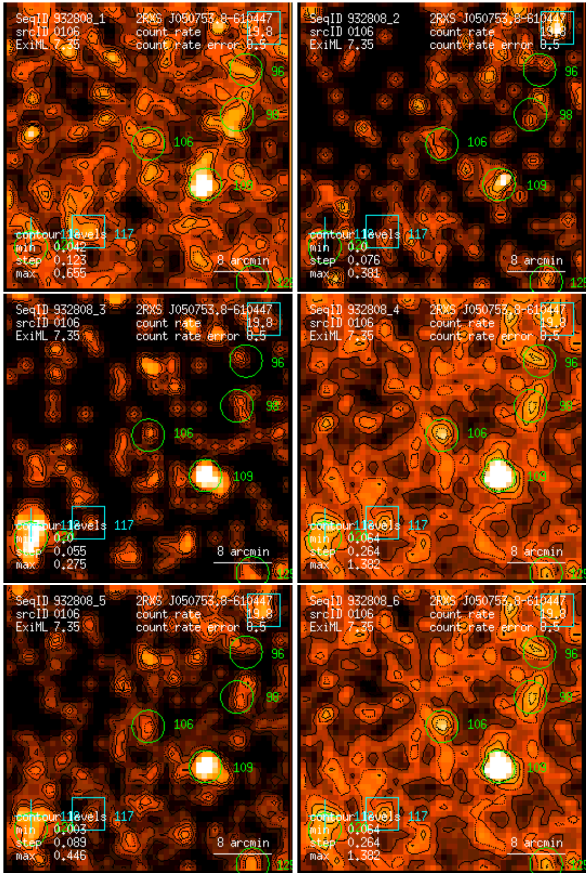
Figure 106: RASS 932808: detection 0106: band rate images, Gaussian filter: (1) PSPC channels 11 – 41, (2) 52 – 90, (3) 91 – 201, (4) 11 – 235, (5) 52 – 201, (6) 11 – 201. Broad band rates in counts/ks. Band rate contour levels in counts/ks/arcmin 2 .
