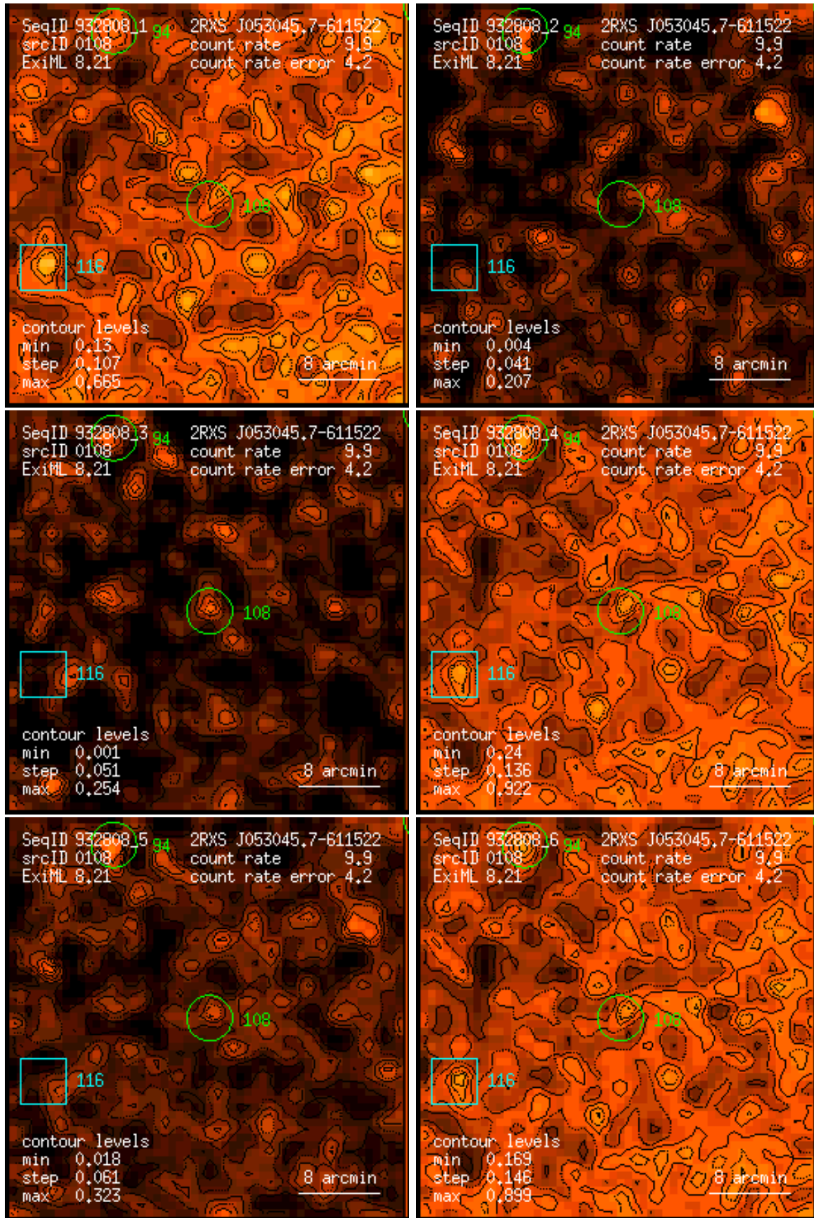
Figure 108: RASS 932808: detection 0108: band rate images, Gaussian filter: (1) PSPC channels 11 – 41, (2) 52 – 90, (3) 91 – 201, (4) 11 – 235, (5) 52 – 201, (6) 11 – 201. Broad band rates in counts/ks. Band rate contour levels in counts/ks/arcmin 2 .
