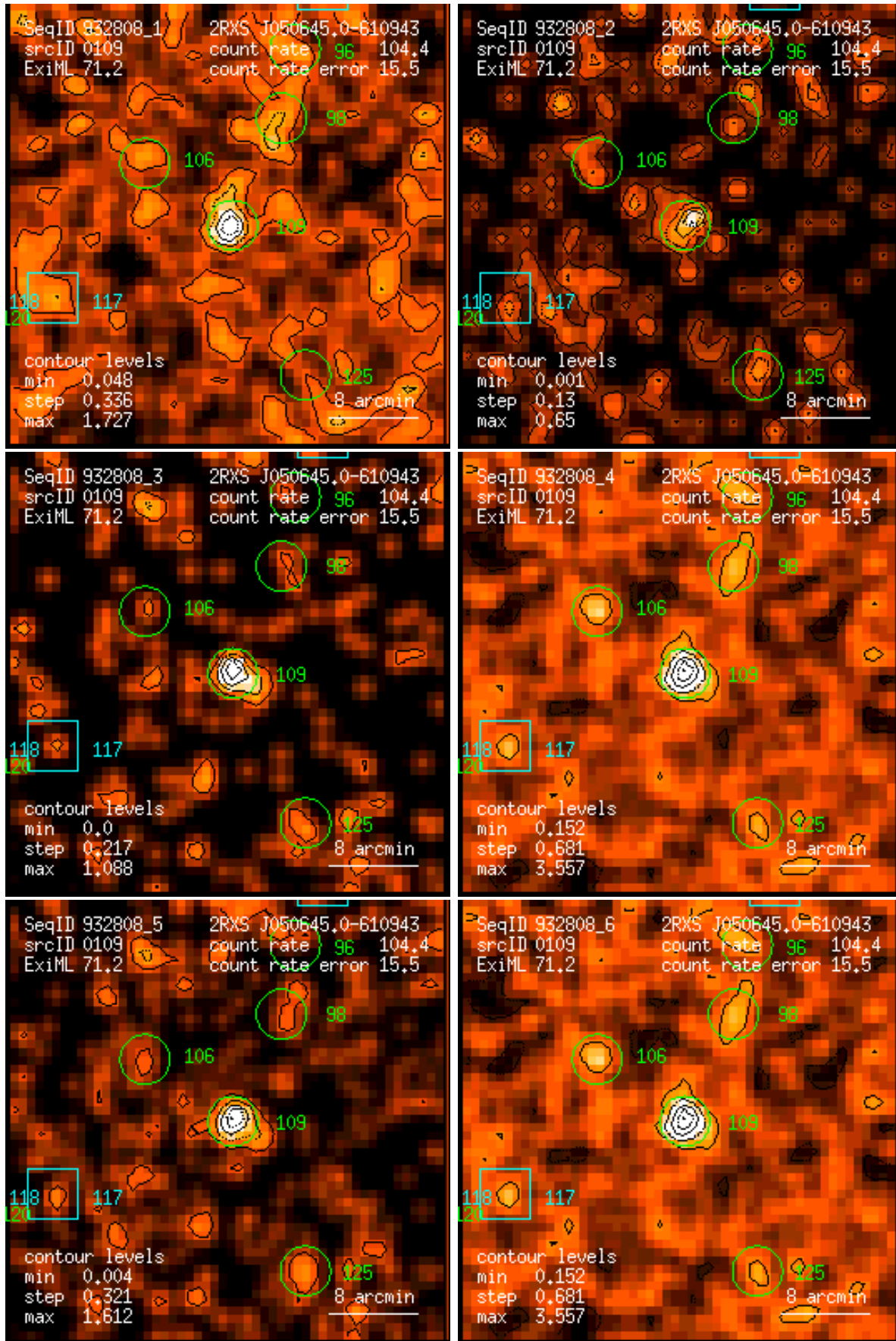
Figure 109: RASS 932808: detection 0109: band rate images, Gaussian filter: (1) PSPC channels 11 – 41, (2) 52 – 90, (3) 91 – 201, (4) 11 – 235, (5) 52 – 201, (6) 11 – 201. Broad band rates in counts/ks. Band rate contour levels in counts/ks/arcmin 2 .
