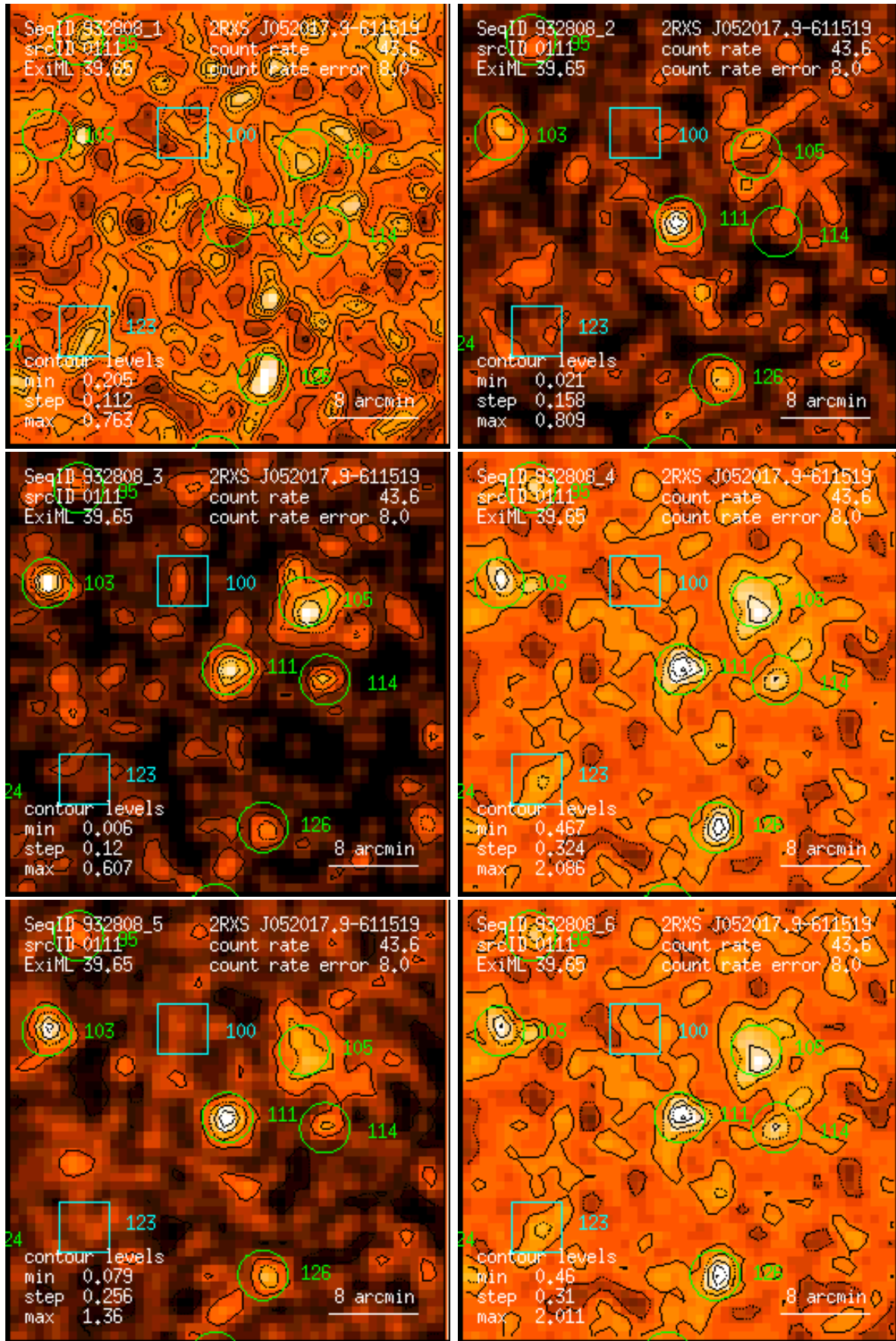
Figure 111: RASS 932808: detection 0111: band rate images, Gaussian filter: (1) PSPC channels 11 – 41, (2) 52 – 90, (3) 91 – 201, (4) 11 – 235, (5) 52 – 201, (6) 11 – 201. Broad band rates in counts/ks. Band rate contour levels in counts/ks/arcmin 2 .
