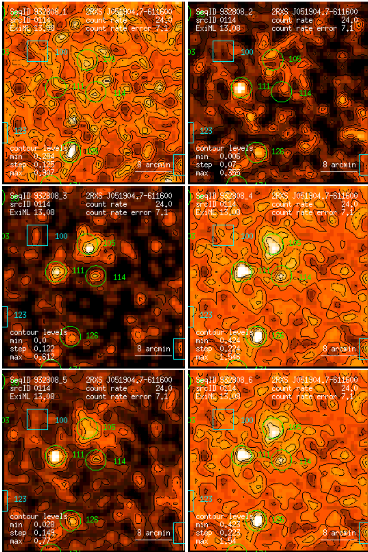
Figure 114: RASS 932808: detection 0114: band rate images, Gaussian filter: (1) PSPC channels 11 – 41, (2) 52 – 90, (3) 91 – 201, (4) 11 – 235, (5) 52 – 201, (6) 11 – 201. Broad band rates in counts/ks. Band rate contour levels in counts/ks/arcmin 2 .
