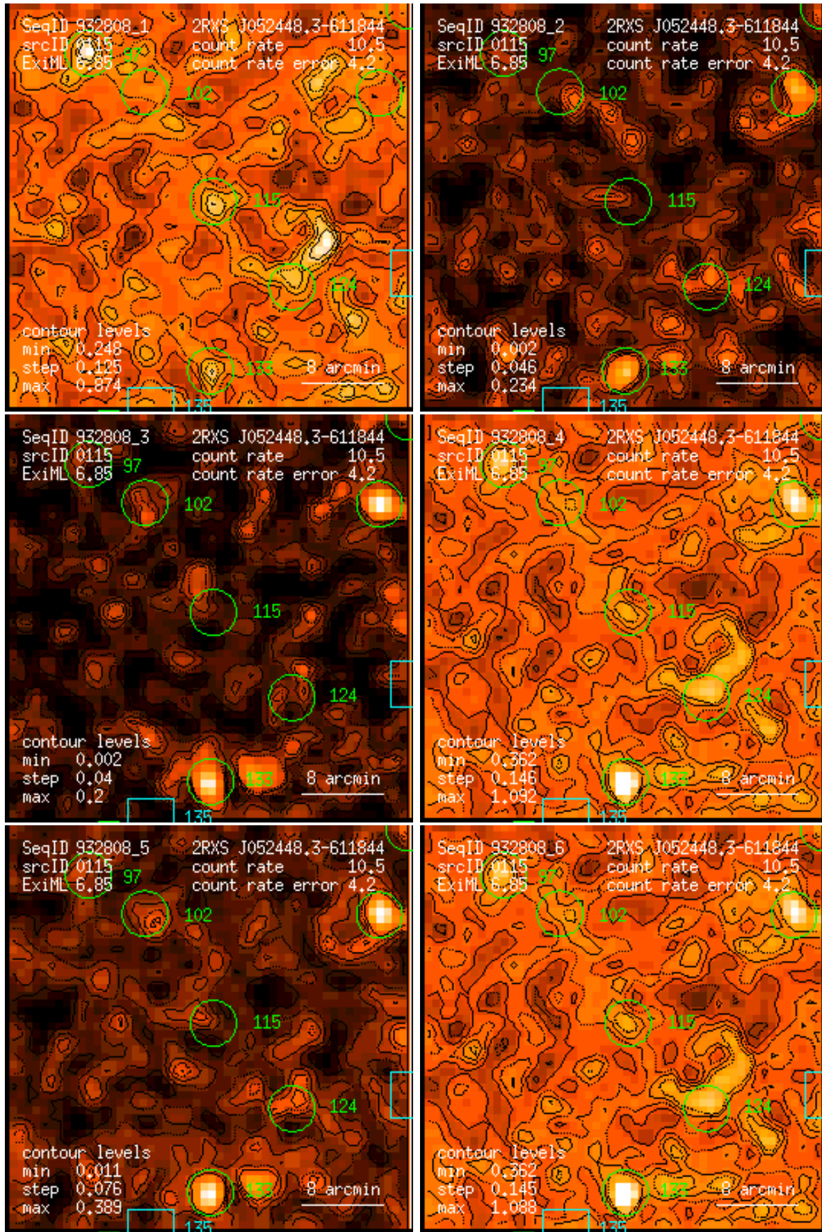
Figure 115: RASS 932808: detection 0115: band rate images, Gaussian filter: (1) PSPC channels 11 – 41, (2) 52 – 90, (3) 91 – 201, (4) 11 – 235, (5) 52 – 201, (6) 11 – 201. Broad band rates in counts/ks. Band rate contour levels in counts/ks/arcmin 2 .
