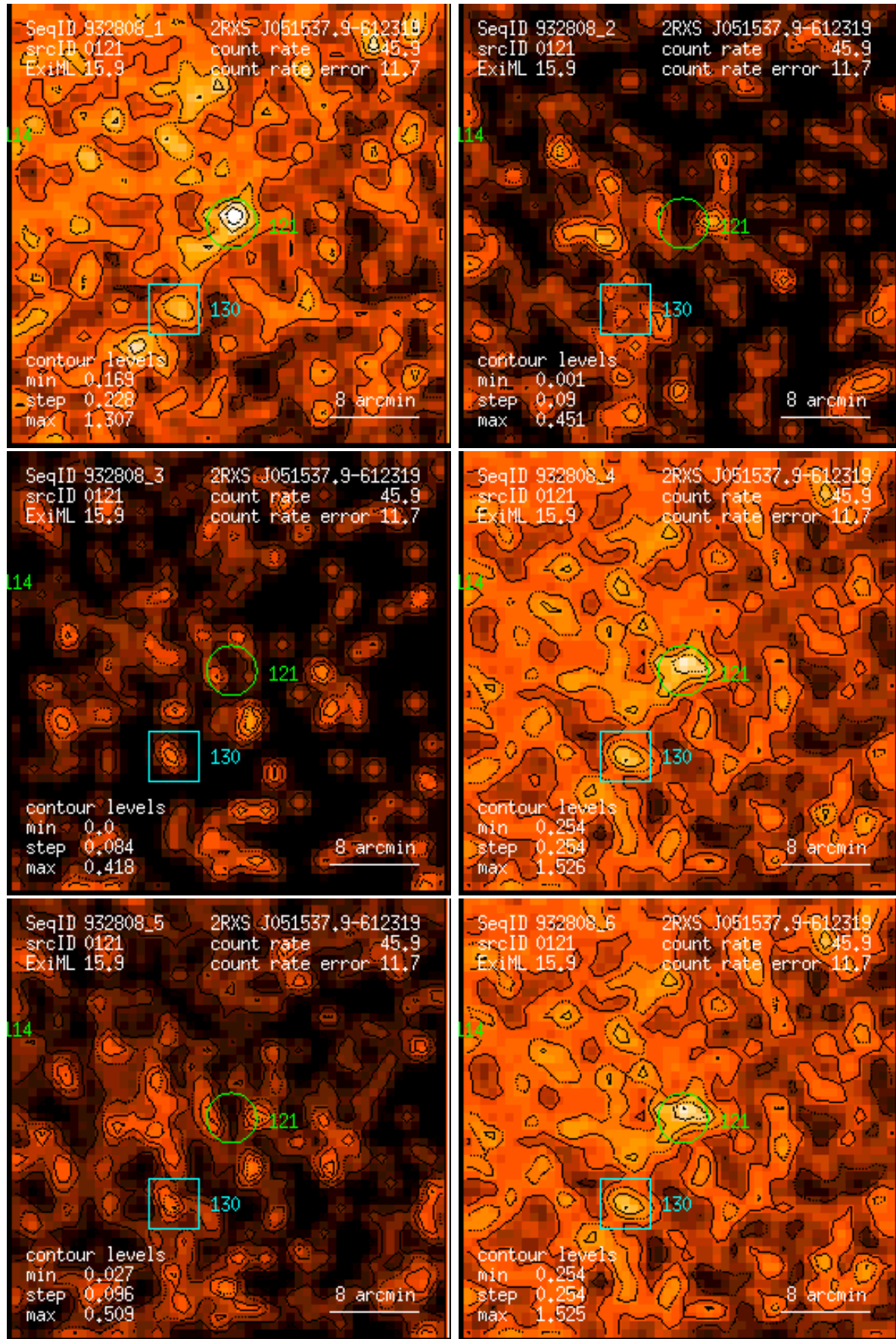
Figure 121: RASS 932808: detection 0121: band rate images, Gaussian filter: (1) PSPC channels 11 – 41, (2) 52 – 90, (3) 91 – 201, (4) 11 – 235, (5) 52 – 201, (6) 11 – 201. Broad band rates in counts/ks. Band rate contour levels in counts/ks/arcmin 2 .
