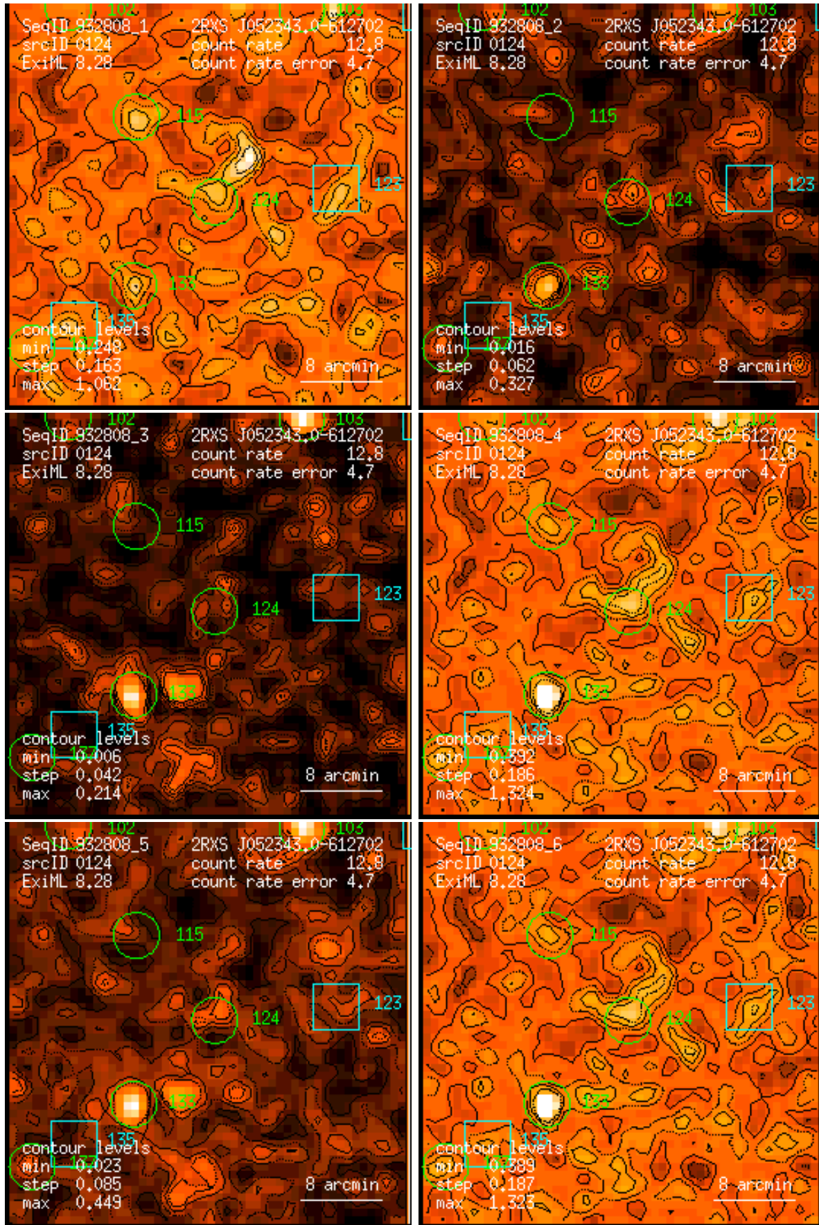
Figure 124: RASS 932808: detection 0124: band rate images, Gaussian filter: (1) PSPC channels 11 – 41, (2) 52 – 90, (3) 91 – 201, (4) 11 – 235, (5) 52 – 201, (6) 11 – 201. Broad band rates in counts/ks. Band rate contour levels in counts/ks/arcmin 2 .
