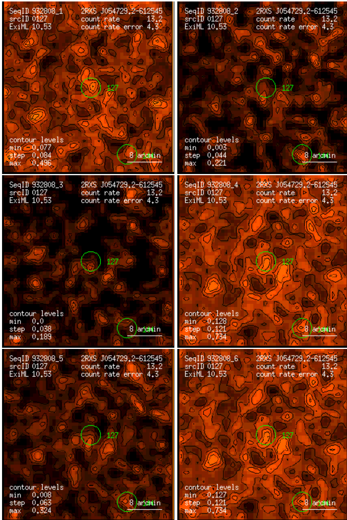
Figure 127: RASS 932808: detection 0127: band rate images, Gaussian filter: (1) PSPC channels 11 – 41, (2) 52 – 90, (3) 91 – 201, (4) 11 – 235, (5) 52 – 201, (6) 11 – 201. Broad band rates in counts/ks. Band rate contour levels in counts/ks/arcmin 2 .
