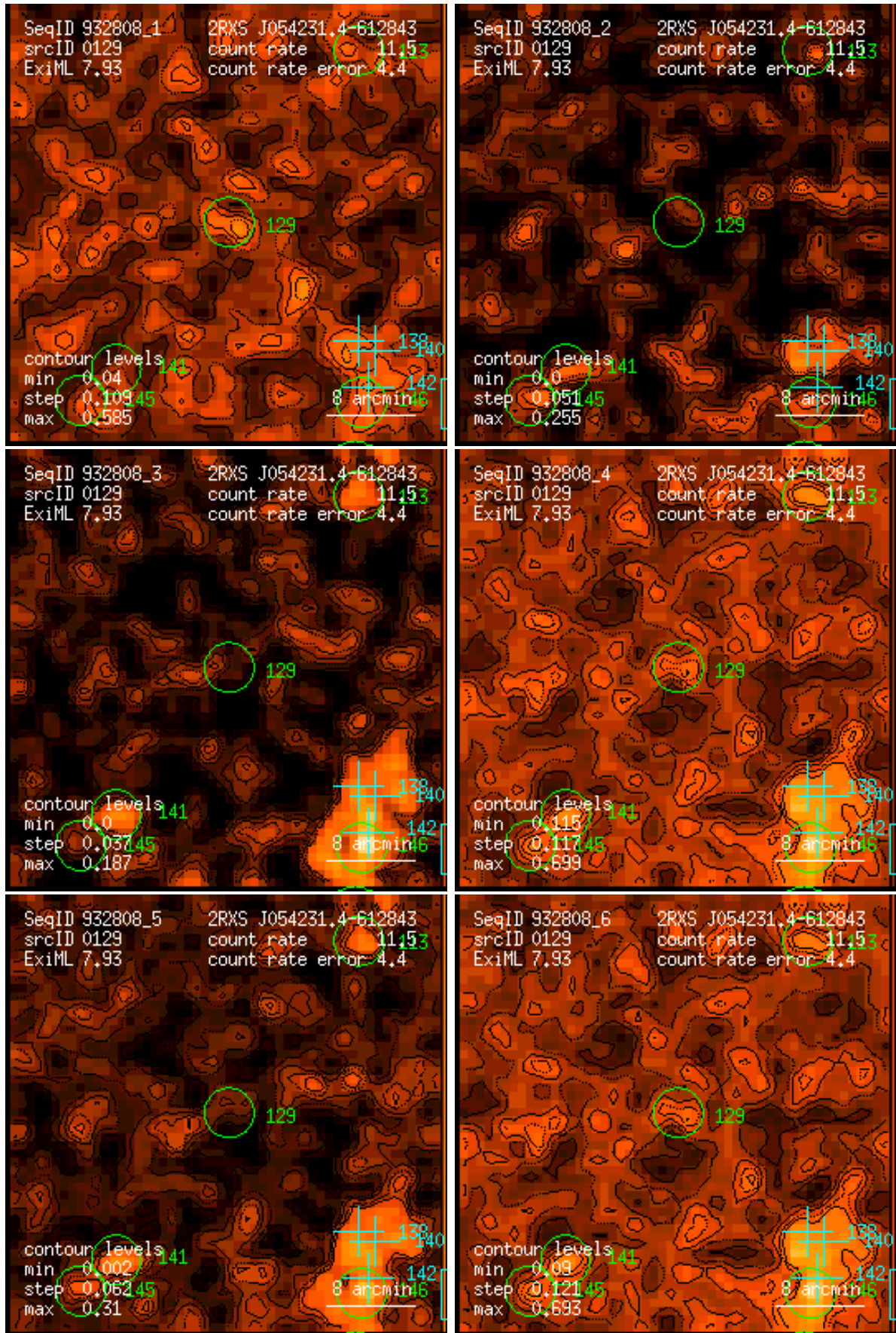
Figure 129: RASS 932808: detection 0129: band rate images, Gaussian filter: (1) PSPC channels 11 – 41, (2) 52 – 90, (3) 91 – 201, (4) 11 – 235, (5) 52 – 201, (6) 11 – 201. Broad band rates in counts/ks. Band rate contour levels in counts/ks/arcmin 2 .
