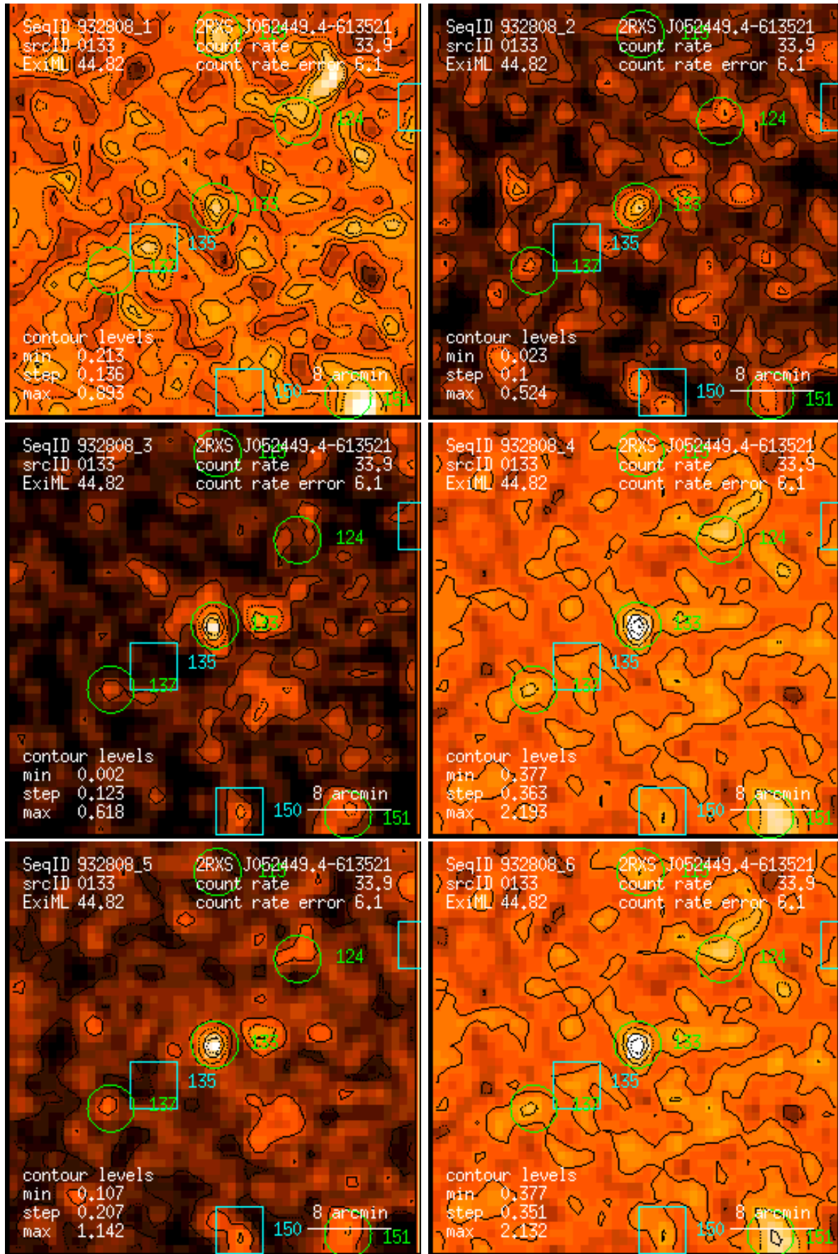
Figure 133: RASS 932808: detection 0133: band rate images, Gaussian filter: (1) PSPC channels 11 – 41, (2) 52 – 90, (3) 91 – 201, (4) 11 – 235, (5) 52 – 201, (6) 11 – 201. Broad band rates in counts/ks. Band rate contour levels in counts/ks/arcmin 2 .
