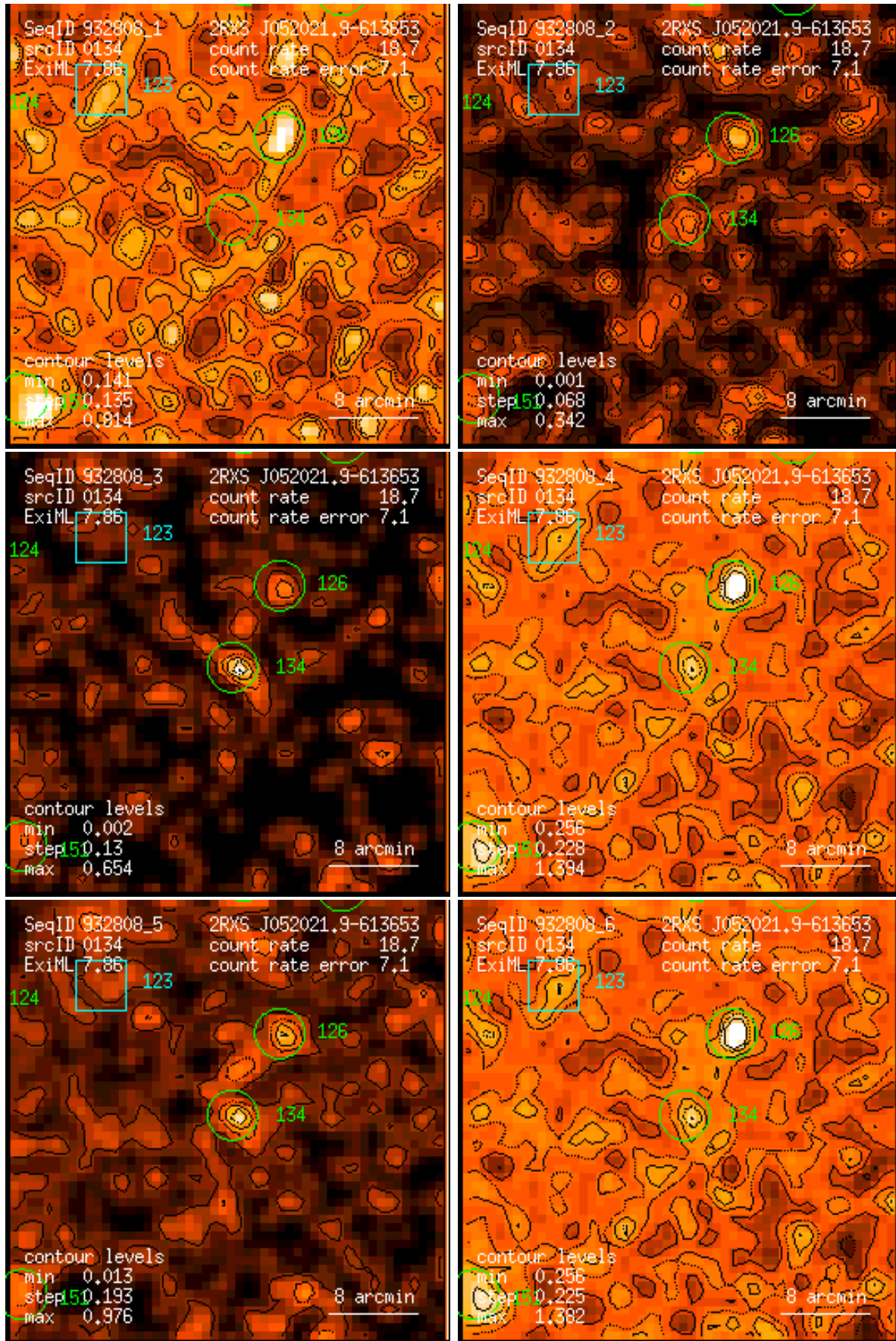
Figure 134: RASS 932808: detection 0134: band rate images, Gaussian filter: (1) PSPC channels 11 – 41, (2) 52 – 90, (3) 91 – 201, (4) 11 – 235, (5) 52 – 201, (6) 11 – 201. Broad band rates in counts/ks. Band rate contour levels in counts/ks/arcmin 2 .
