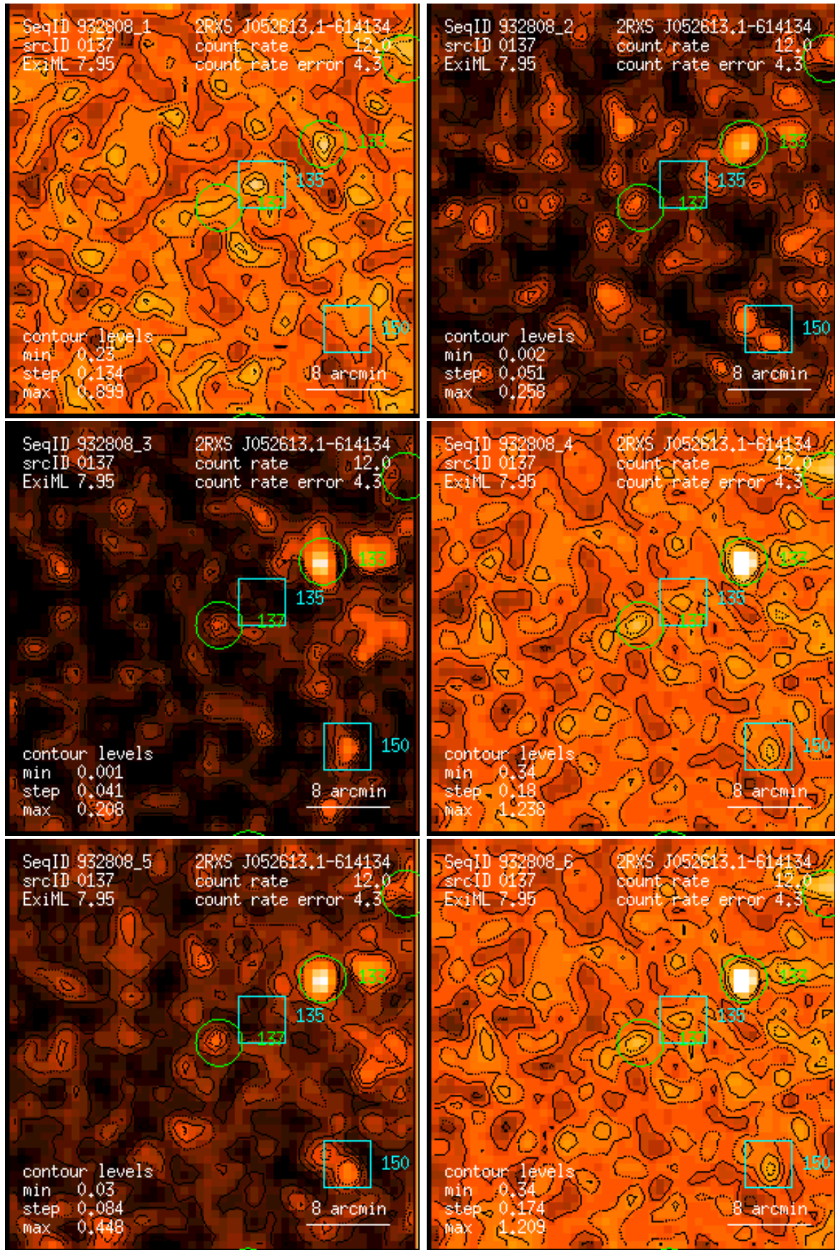
Figure 137: RASS 932808: detection 0137: band rate images, Gaussian filter: (1) PSPC channels 11 – 41, (2) 52 – 90, (3) 91 – 201, (4) 11 – 235, (5) 52 – 201, (6) 11 – 201. Broad band rates in counts/ks. Band rate contour levels in counts/ks/arcmin 2 .
