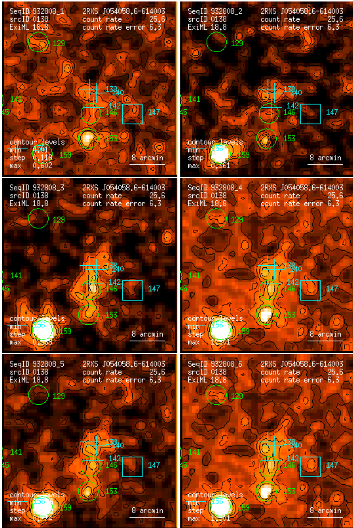
Figure 138: RASS 932808: detection 0138: band rate images, Gaussian filter: (1) PSPC channels 11 – 41, (2) 52 – 90, (3) 91 – 201, (4) 11 – 235, (5) 52 – 201, (6) 11 – 201. Broad band rates in counts/ks. Band rate contour levels in counts/ks/arcmin 2 .
