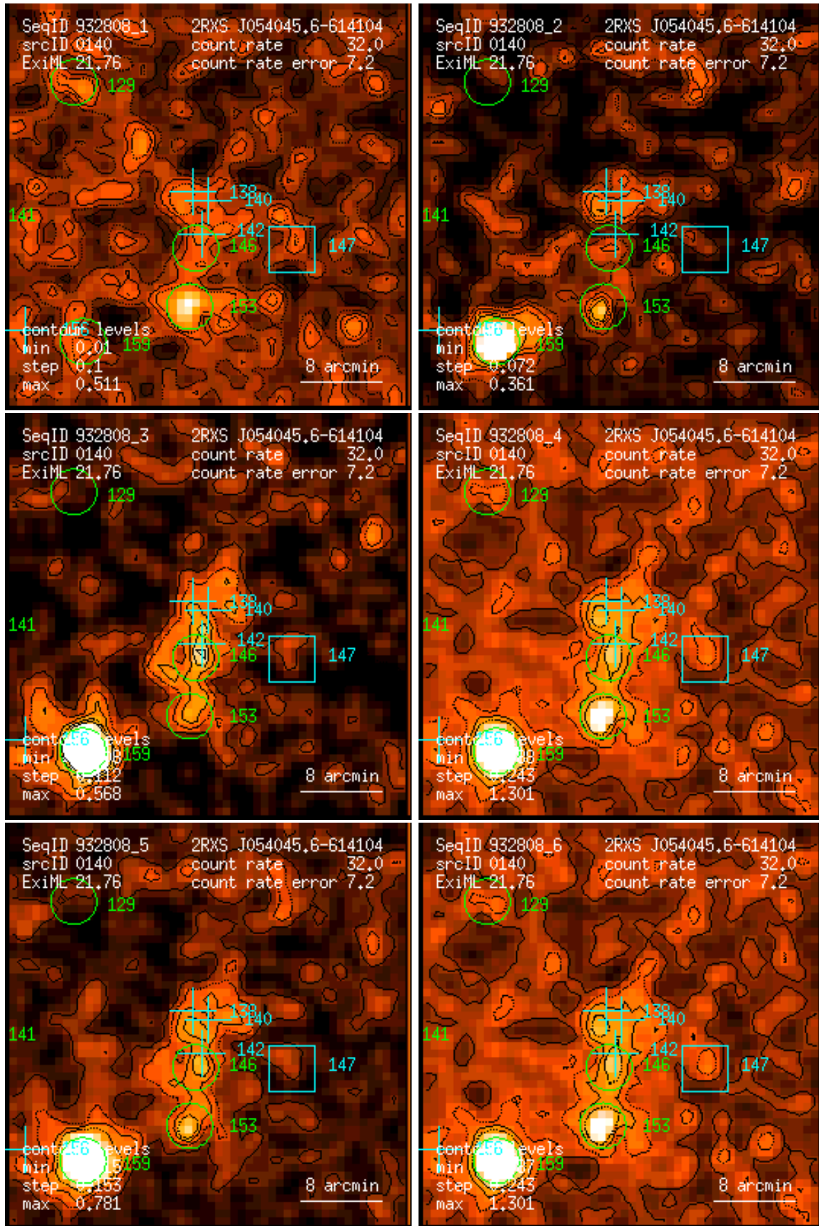
Figure 140: RASS 932808: detection 0140: band rate images, Gaussian filter: (1) PSPC channels 11 – 41, (2) 52 – 90, (3) 91 – 201, (4) 11 – 235, (5) 52 – 201, (6) 11 – 201. Broad band rates in counts/ks. Band rate contour levels in counts/ks/arcmin 2 .
