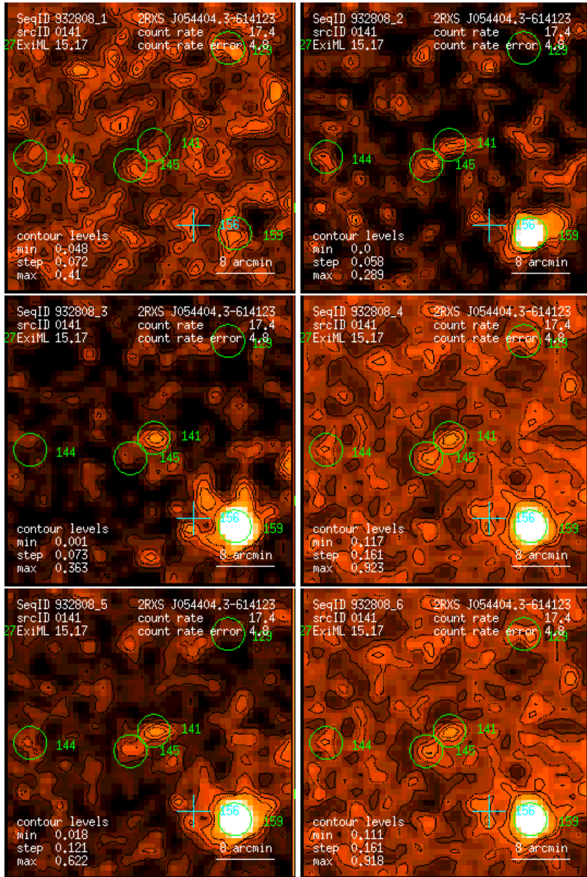
Figure 141: RASS 932808: detection 0141: band rate images, Gaussian filter: (1) PSPC channels 11 – 41, (2) 52 – 90, (3) 91 – 201, (4) 11 – 235, (5) 52 – 201, (6) 11 – 201. Broad band rates in counts/ks. Band rate contour levels in counts/ks/arcmin 2 .
