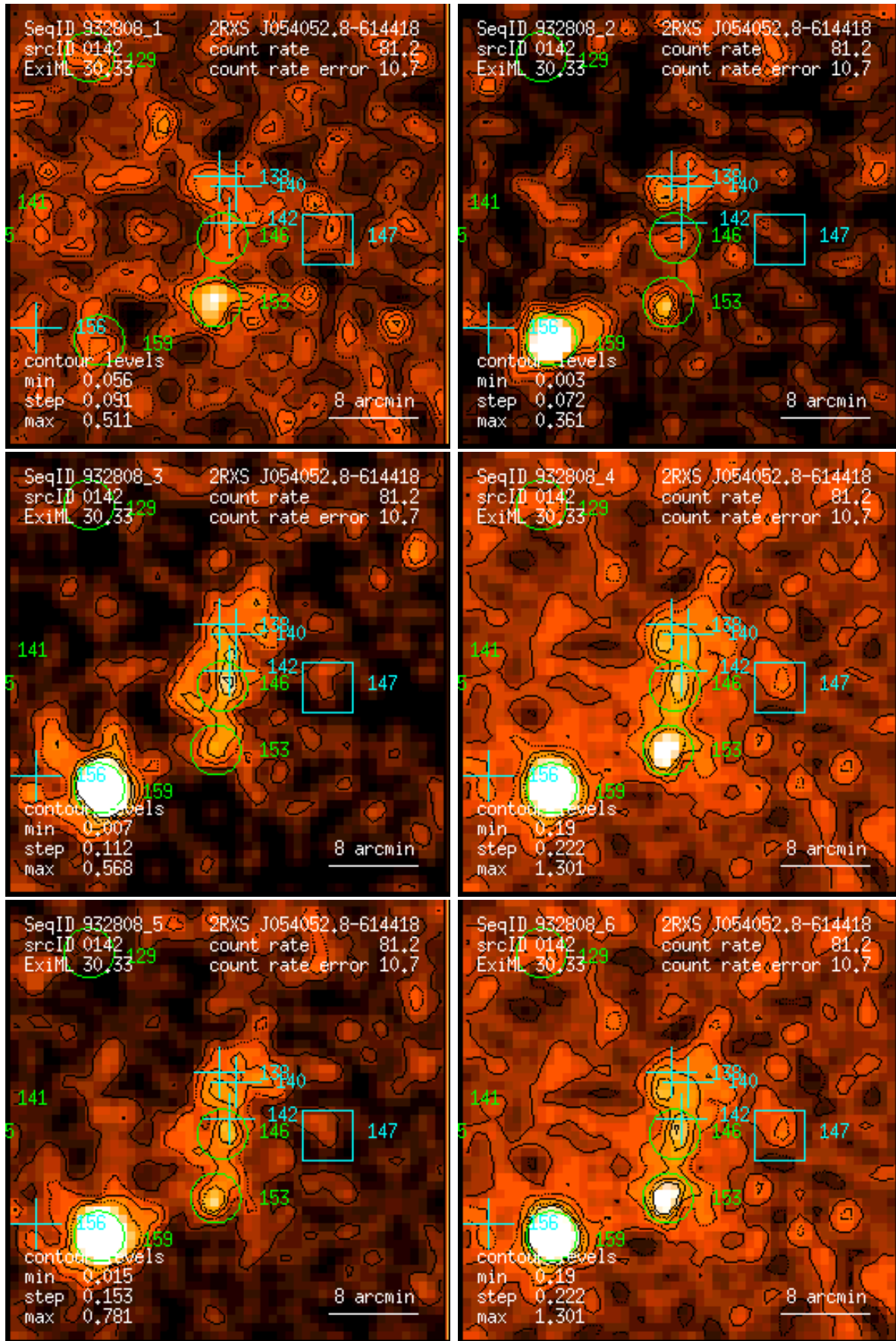
Figure 142: RASS 932808: detection 0142: band rate images, Gaussian filter: (1) PSPC channels 11 – 41, (2) 52 – 90, (3) 91 – 201, (4) 11 – 235, (5) 52 – 201, (6) 11 – 201. Broad band rates in counts/ks. Band rate contour levels in counts/ks/arcmin 2 .
