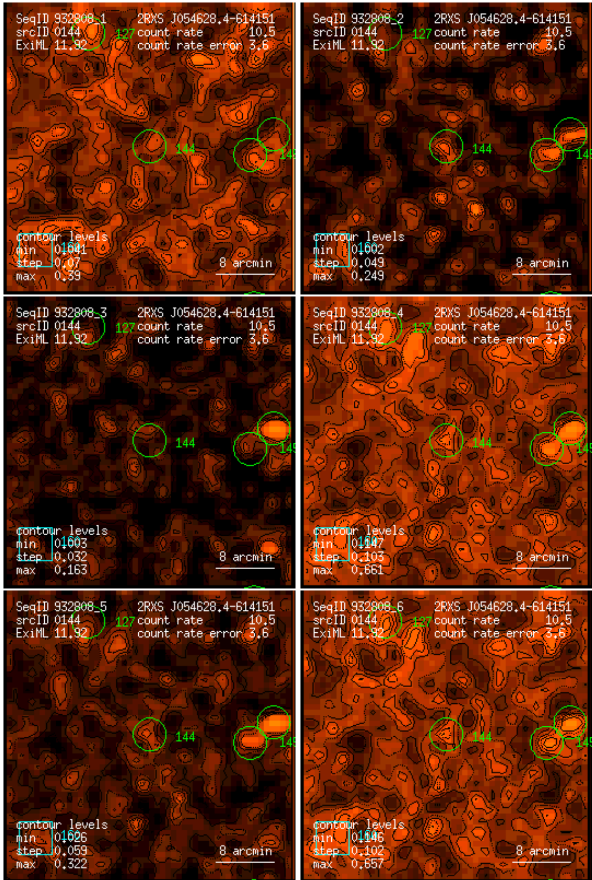
Figure 144: RASS 932808: detection 0144: band rate images, Gaussian filter: (1) PSPC channels 11 – 41, (2) 52 – 90, (3) 91 – 201, (4) 11 – 235, (5) 52 – 201, (6) 11 – 201. Broad band rates in counts/ks. Band rate contour levels in counts/ks/arcmin 2 .
