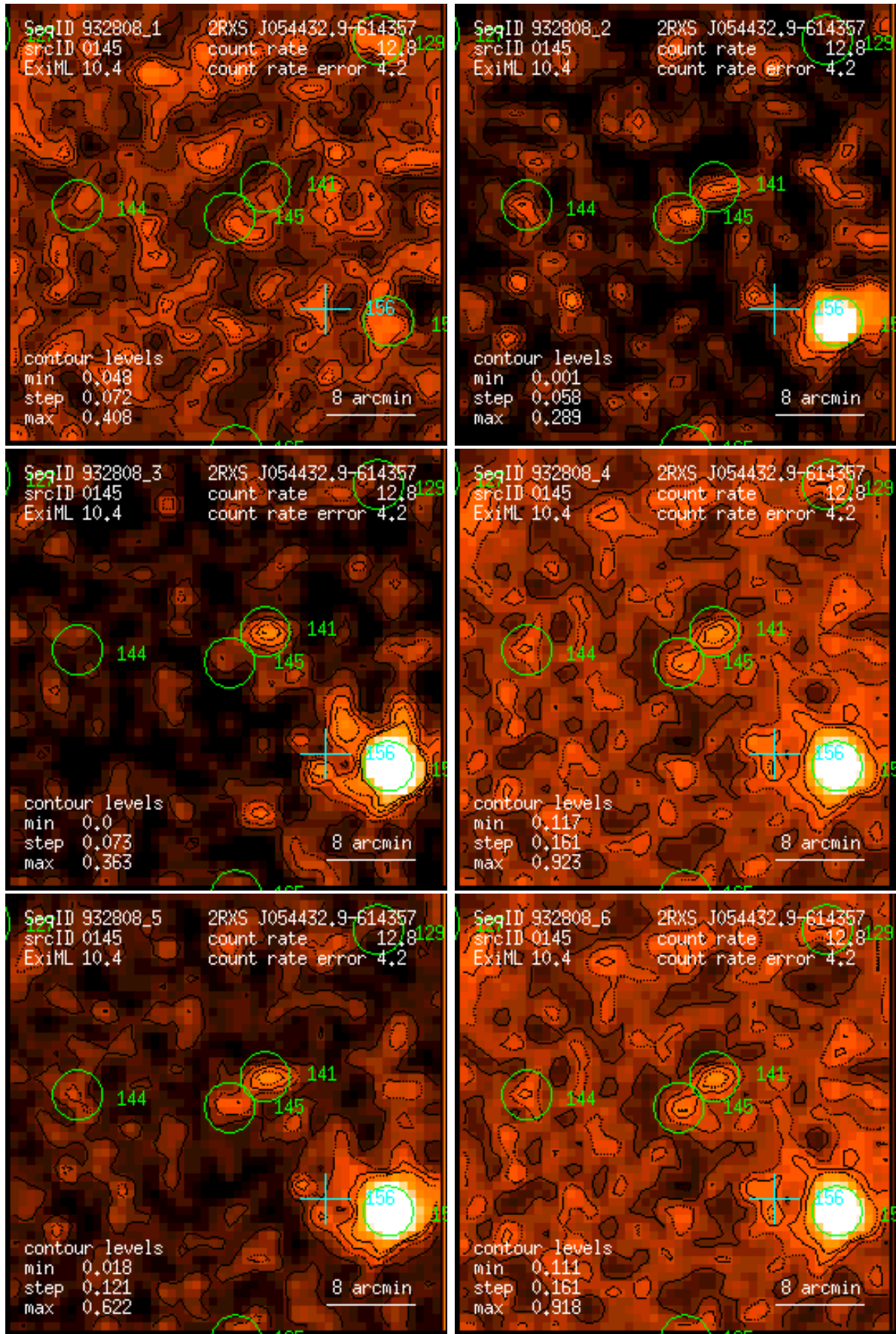
Figure 145: RASS 932808: detection 0145: band rate images, Gaussian filter: (1) PSPC channels 11 – 41, (2) 52 – 90, (3) 91 – 201, (4) 11 – 235, (5) 52 – 201, (6) 11 – 201. Broad band rates in counts/ks. Band rate contour levels in counts/ks/arcmin 2 .
