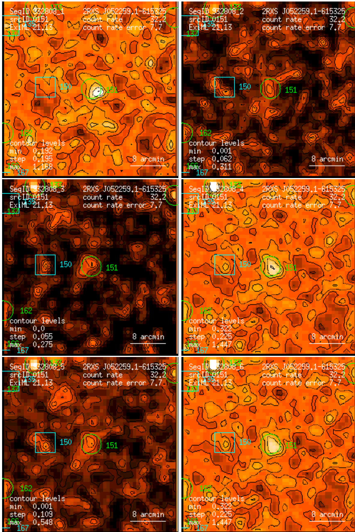
Figure 151: RASS 932808: detection 0151: band rate images, Gaussian filter: (1) PSPC channels 11 – 41, (2) 52 – 90, (3) 91 – 201, (4) 11 – 235, (5) 52 – 201, (6) 11 – 201. Broad band rates in counts/ks. Band rate contour levels in counts/ks/arcmin 2 .
