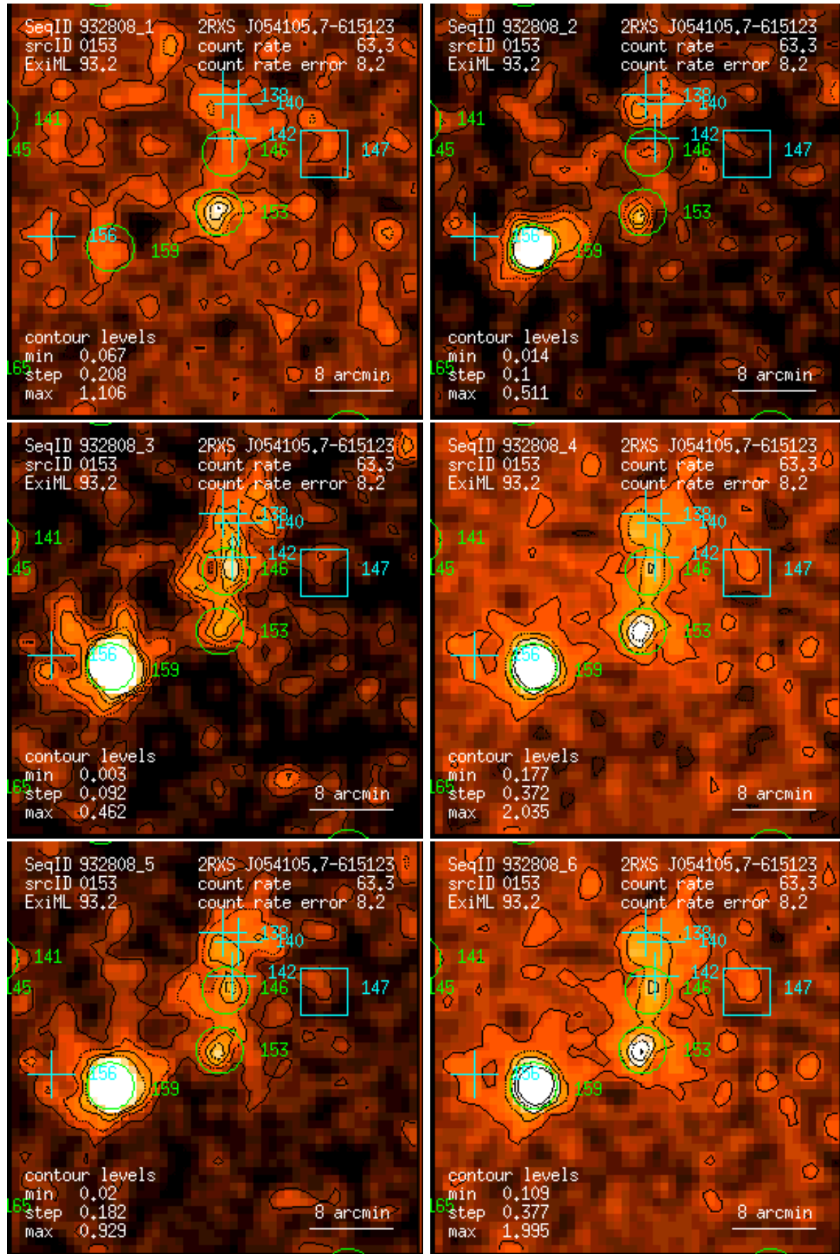
Figure 153: RASS 932808: detection 0153: band rate images, Gaussian filter: (1) PSPC channels 11 – 41, (2) 52 – 90, (3) 91 – 201, (4) 11 – 235, (5) 52 – 201, (6) 11 – 201. Broad band rates in counts/ks. Band rate contour levels in counts/ks/arcmin 2 .
