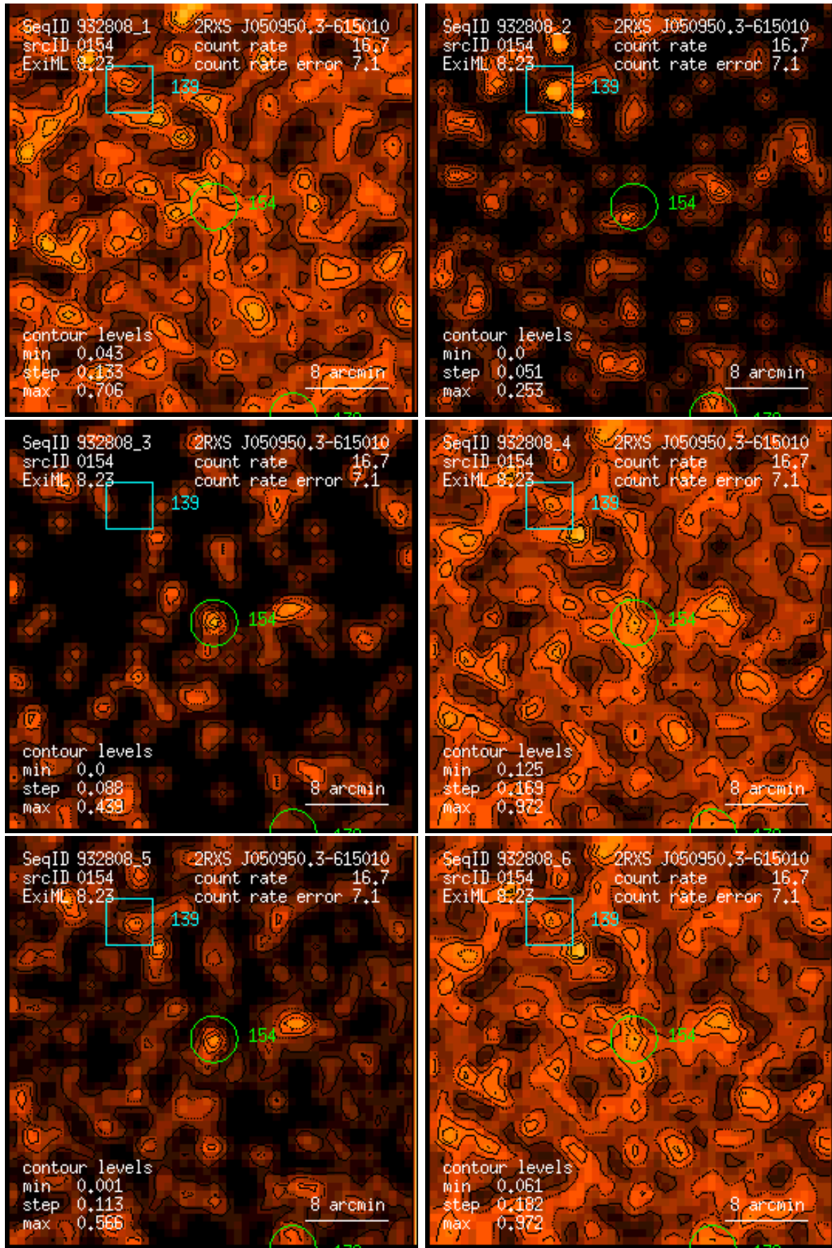
Figure 154: RASS 932808: detection 0154: band rate images, Gaussian filter: (1) PSPC channels 11 – 41, (2) 52 – 90, (3) 91 – 201, (4) 11 – 235, (5) 52 – 201, (6) 11 – 201. Broad band rates in counts/ks. Band rate contour levels in counts/ks/arcmin 2 .
