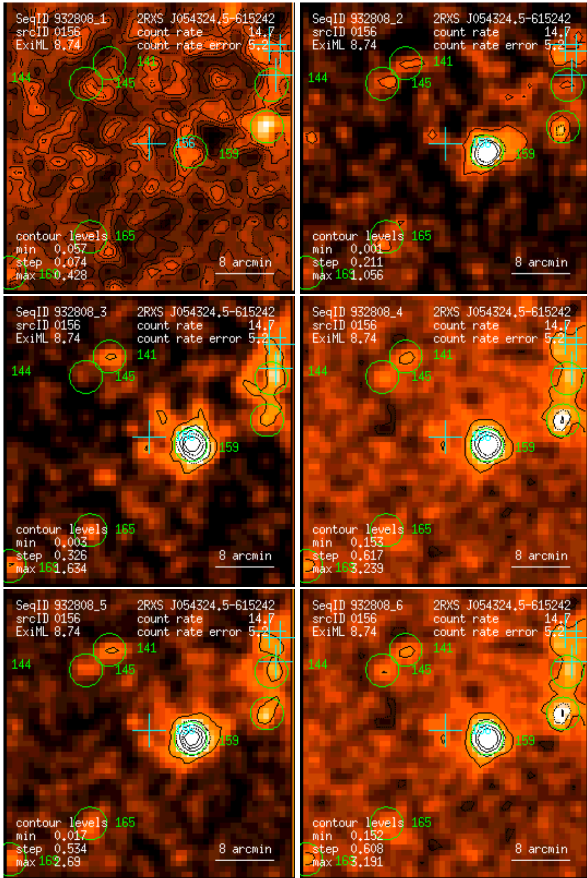
Figure 156: RASS 932808: detection 0156: band rate images, Gaussian filter: (1) PSPC channels 11 – 41, (2) 52 – 90, (3) 91 – 201, (4) 11 – 235, (5) 52 – 201, (6) 11 – 201. Broad band rates in counts/ks. Band rate contour levels in counts/ks/arcmin 2 .
