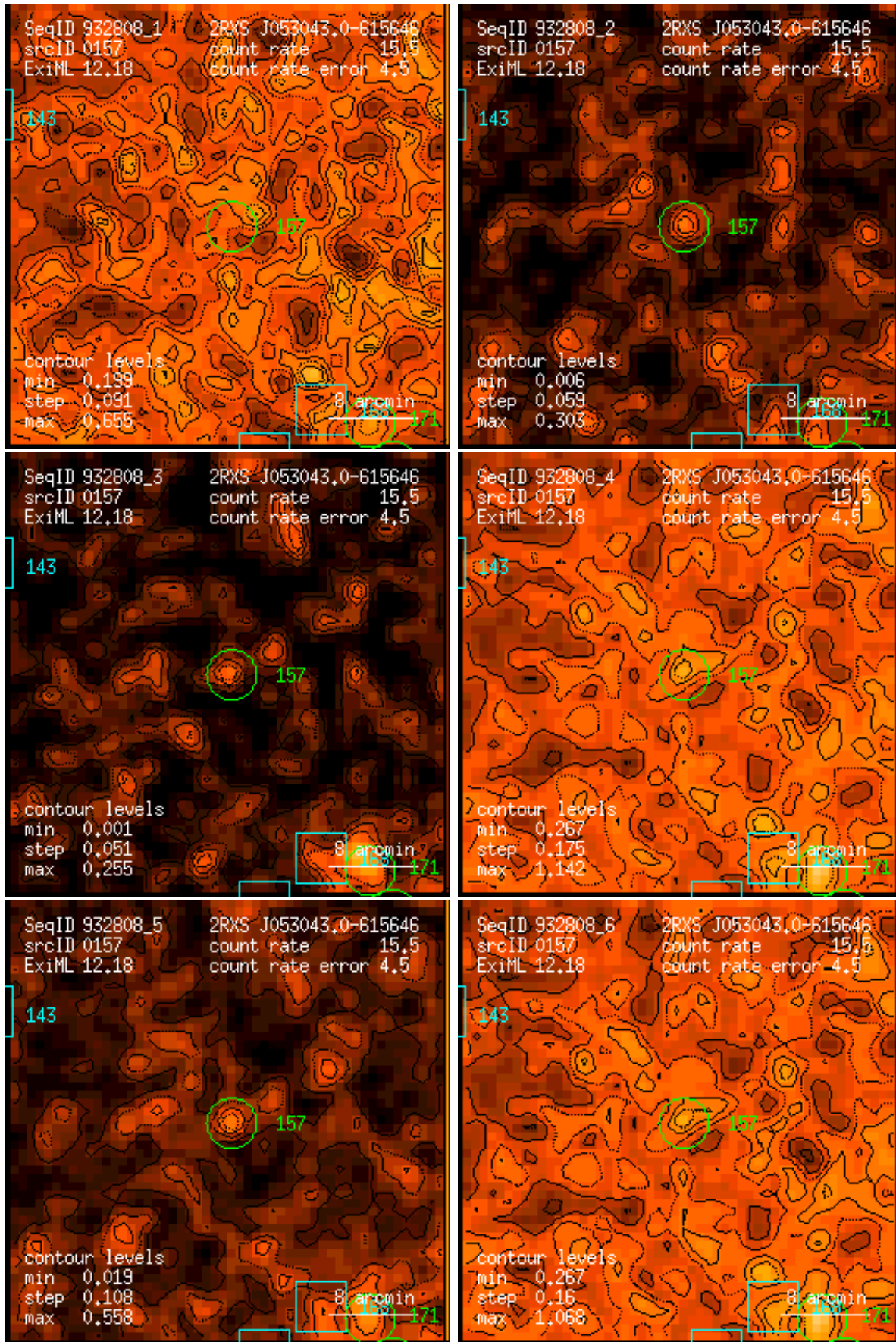
Figure 157: RASS 932808: detection 0157: band rate images, Gaussian filter: (1) PSPC channels 11 – 41, (2) 52 – 90, (3) 91 – 201, (4) 11 – 235, (5) 52 – 201, (6) 11 – 201. Broad band rates in counts/ks. Band rate contour levels in counts/ks/arcmin 2 .
