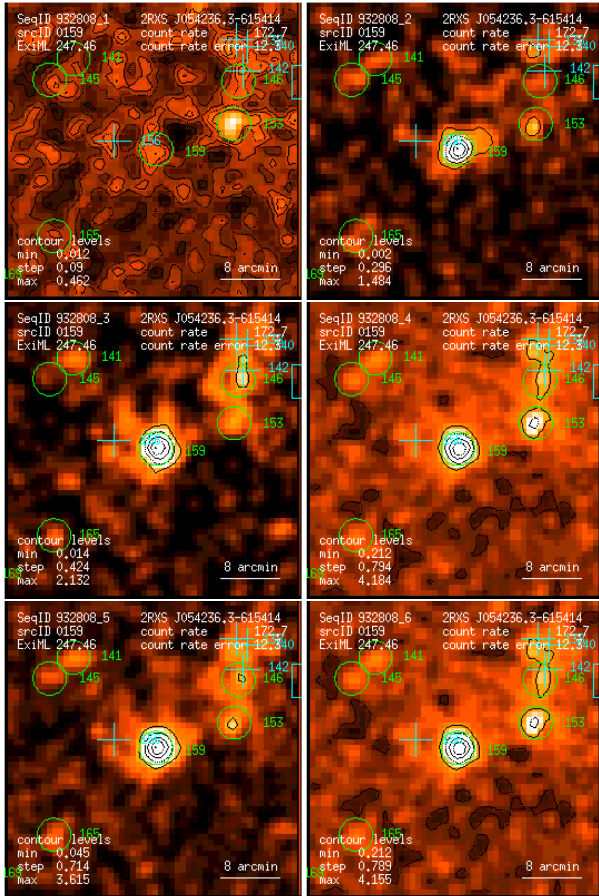
Figure 159: RASS 932808: detection 0159: band rate images, Gaussian filter: (1) PSPC channels 11 – 41, (2) 52 – 90, (3) 91 – 201, (4) 11 – 235, (5) 52 – 201, (6) 11 – 201. Broad band rates in counts/ks. Band rate contour levels in counts/ks/arcmin 2 .
