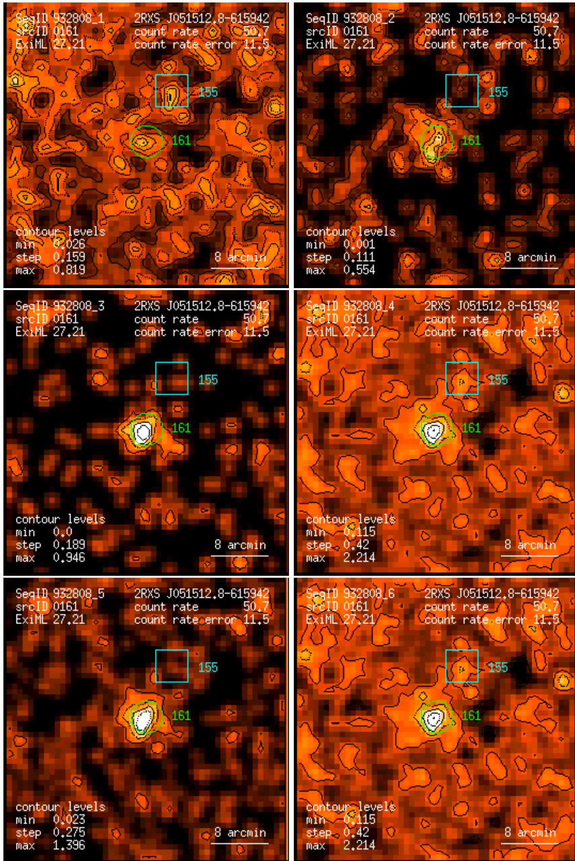
Figure 161: RASS 932808: detection 0161: band rate images, Gaussian filter: (1) PSPC channels 11 – 41, (2) 52 – 90, (3) 91 – 201, (4) 11 – 235, (5) 52 – 201, (6) 11 – 201. Broad band rates in counts/ks. Band rate contour levels in counts/ks/arcmin 2 .
