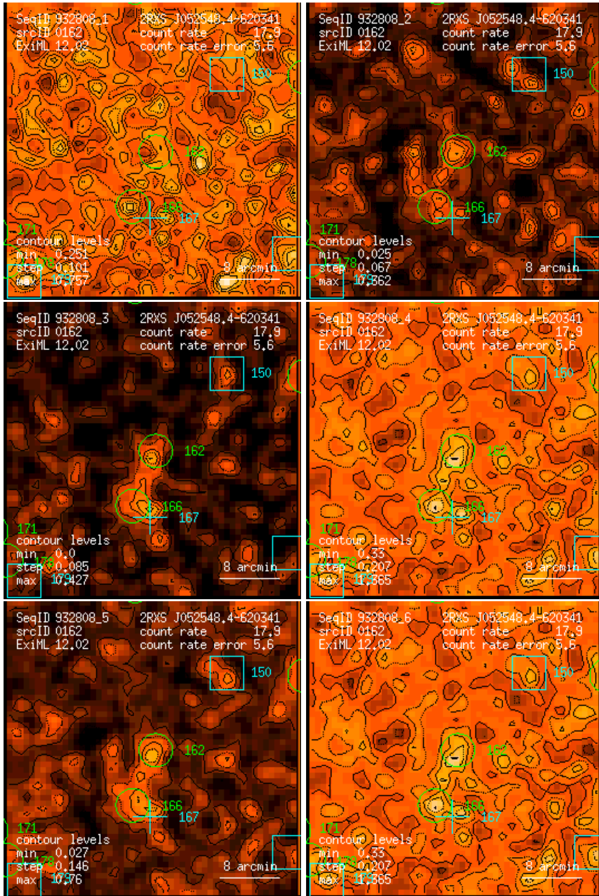
Figure 162: RASS 932808: detection 0162: band rate images, Gaussian filter: (1) PSPC channels 11 – 41, (2) 52 – 90, (3) 91 – 201, (4) 11 – 235, (5) 52 – 201, (6) 11 – 201. Broad band rates in counts/ks. Band rate contour levels in counts/ks/arcmin 2 .
