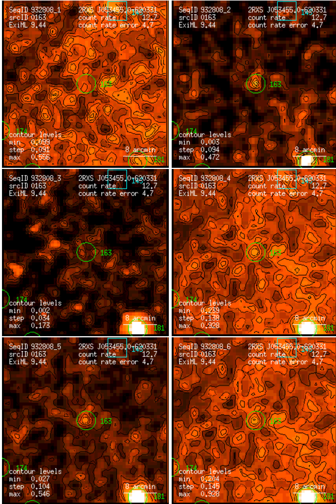
Figure 163: RASS 932808: detection 0163: band rate images, Gaussian filter: (1) PSPC channels 11 – 41, (2) 52 – 90, (3) 91 – 201, (4) 11 – 235, (5) 52 – 201, (6) 11 – 201. Broad band rates in counts/ks. Band rate contour levels in counts/ks/arcmin 2 .
